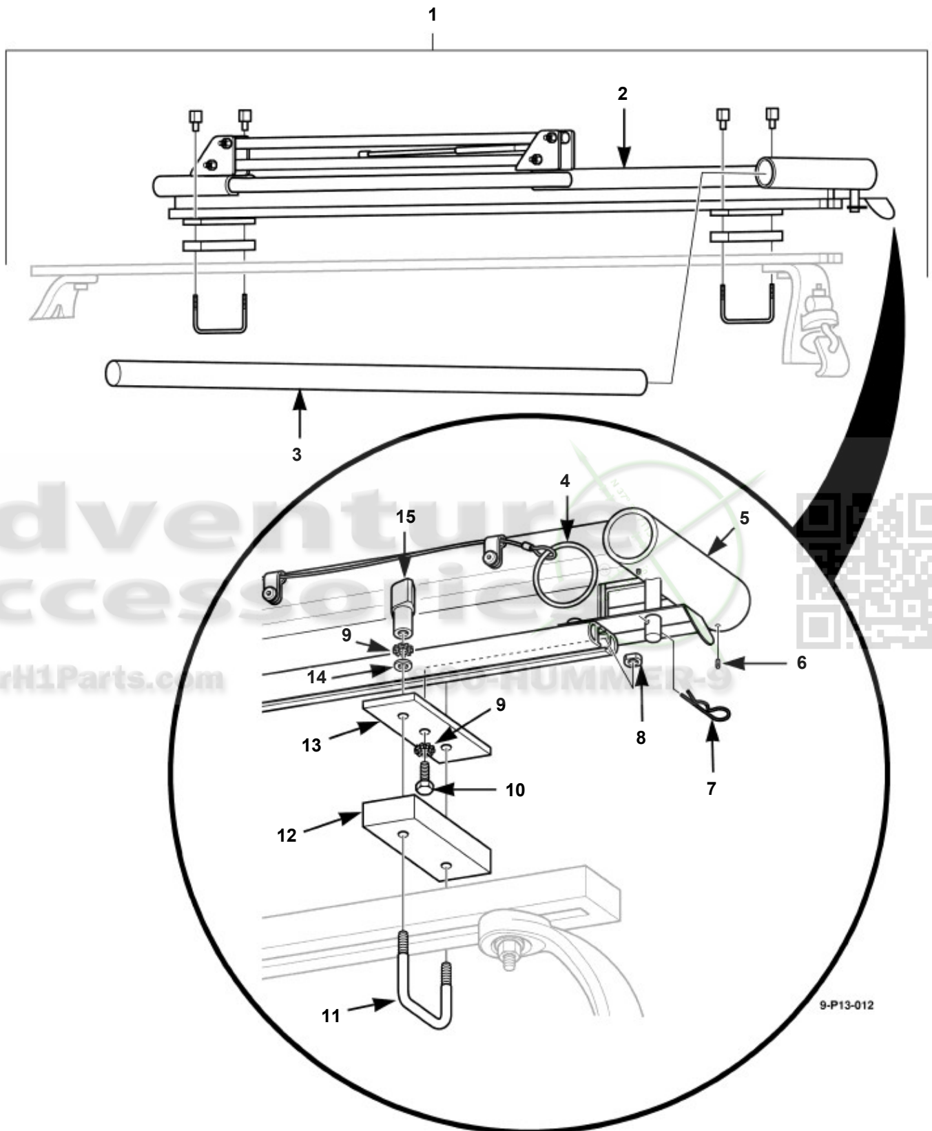
Roof Rack Kit, Side Load
