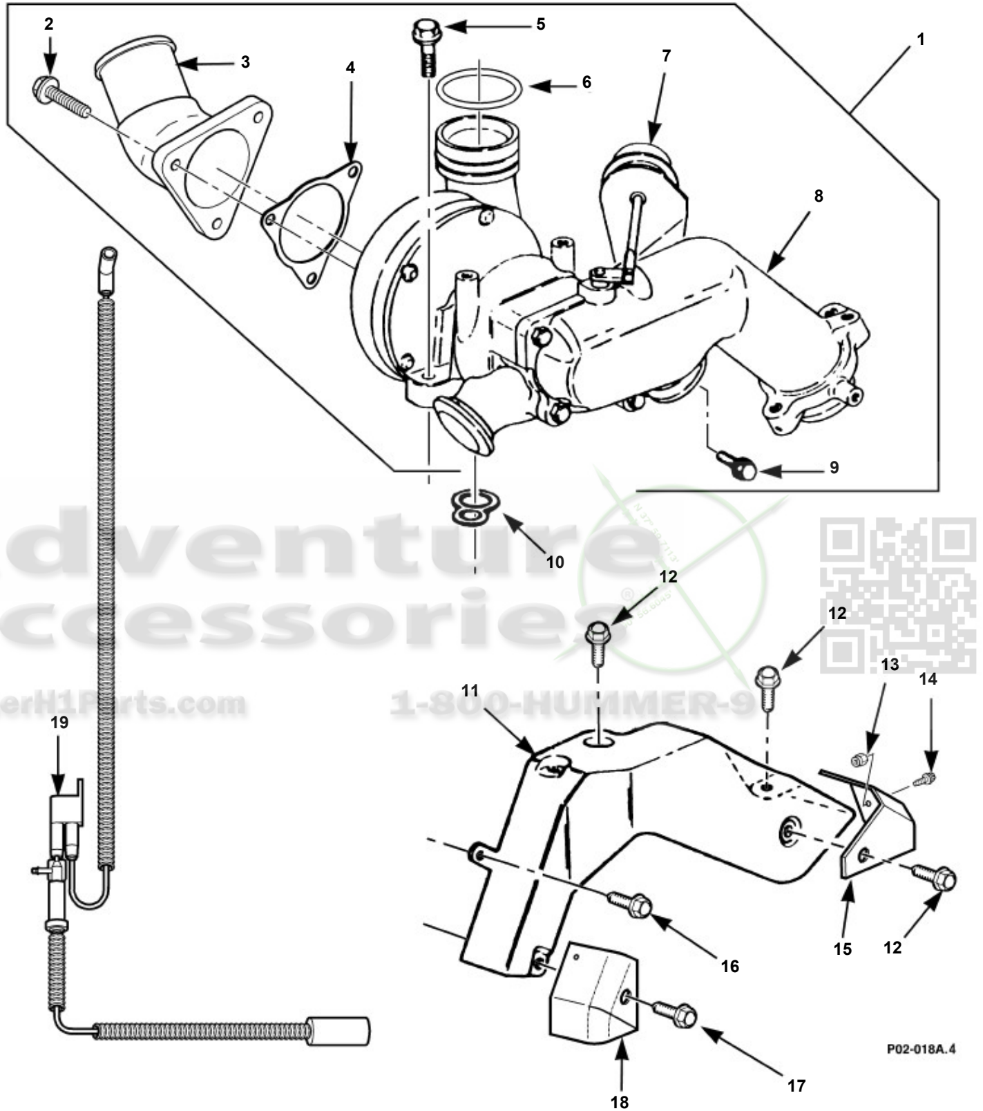
TurboCharger Assembly
