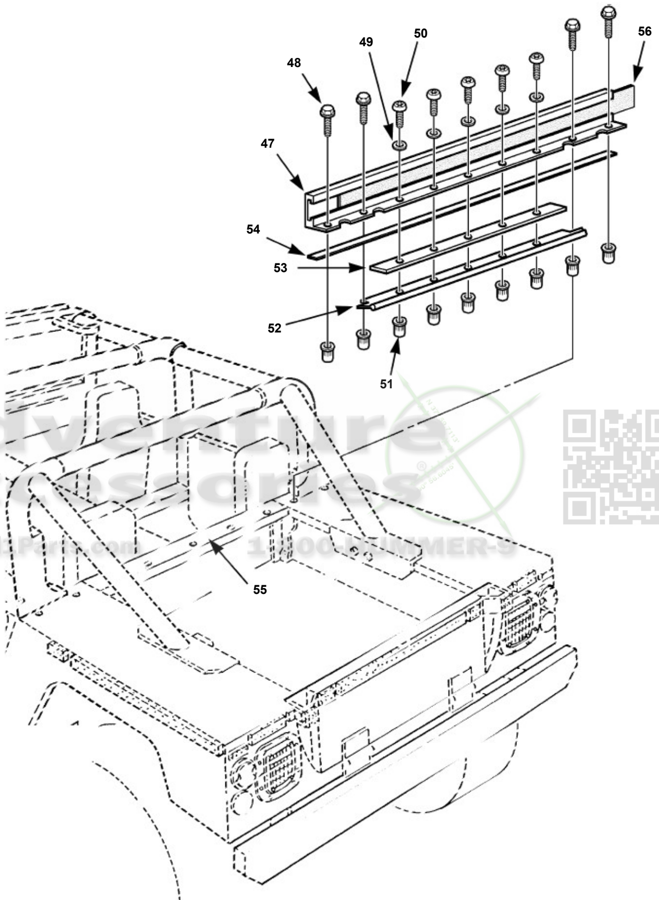
Soft Top Support Structure, Model 90
