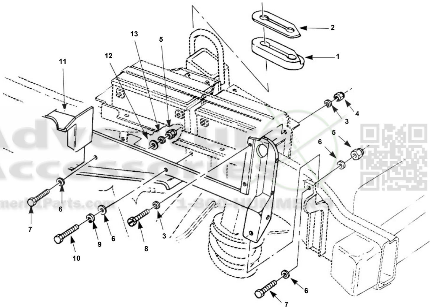
Splash Shield, Right Hand Lower
