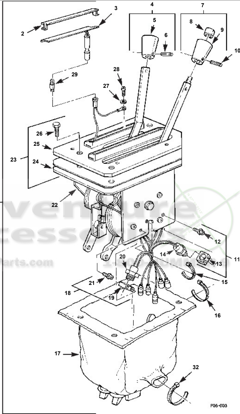
Transmission and Transfer Case Control Assembly and Neutral Start Switch
