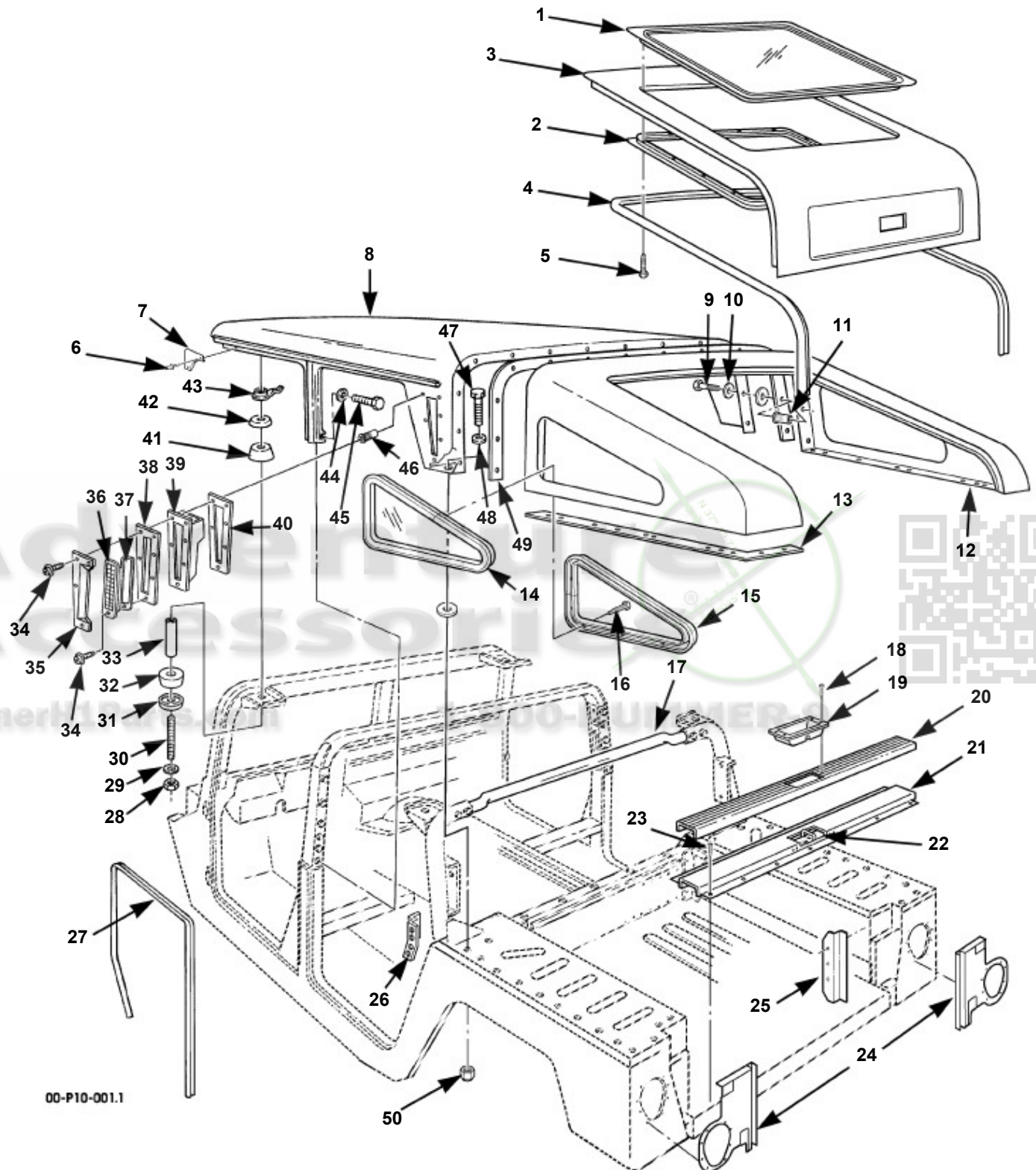
Roof, Slant-Back Door, and Mounting Hardware, SlantBack, Model 90
