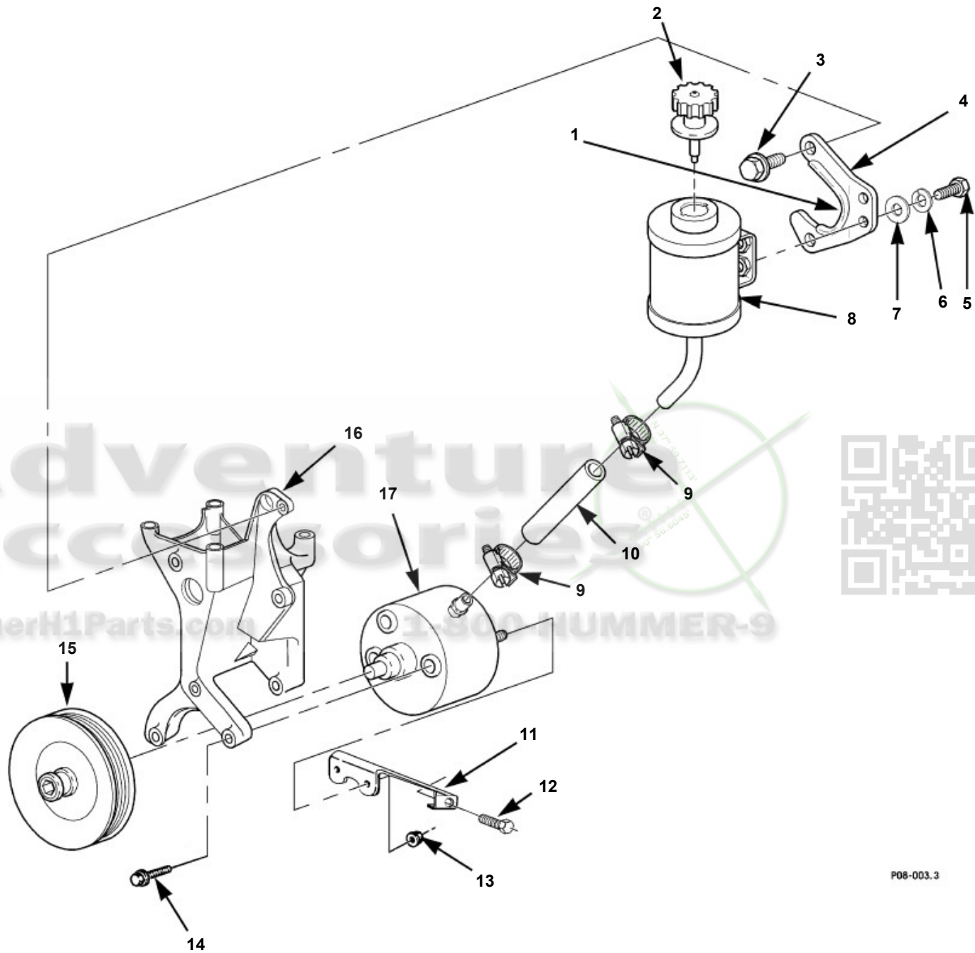
Power Steering Pump, Pulley, Reservoir, and Mounting Hardware
