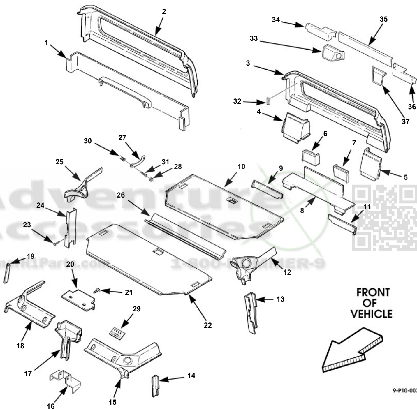
Headliner, Roof Trim, Front and Rear Side Trim, Grab Handles, and Mounting Hardware (Delco Standard Stereo System)
