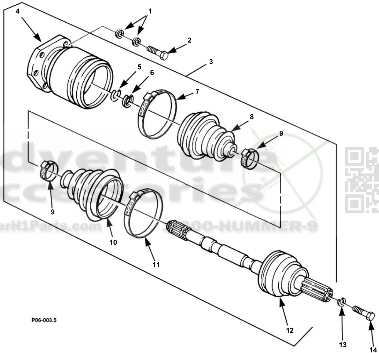
Halfshaft Assembly, Left and Right Side
