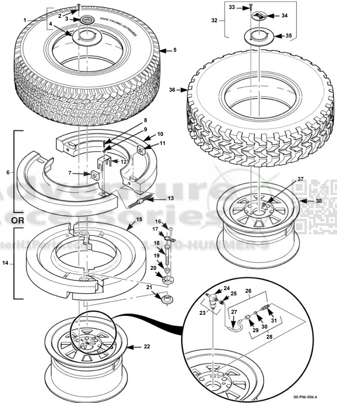
Wheel, Tire and Runflat Assembly, One-Piece Aluminum Rim (Optional)
