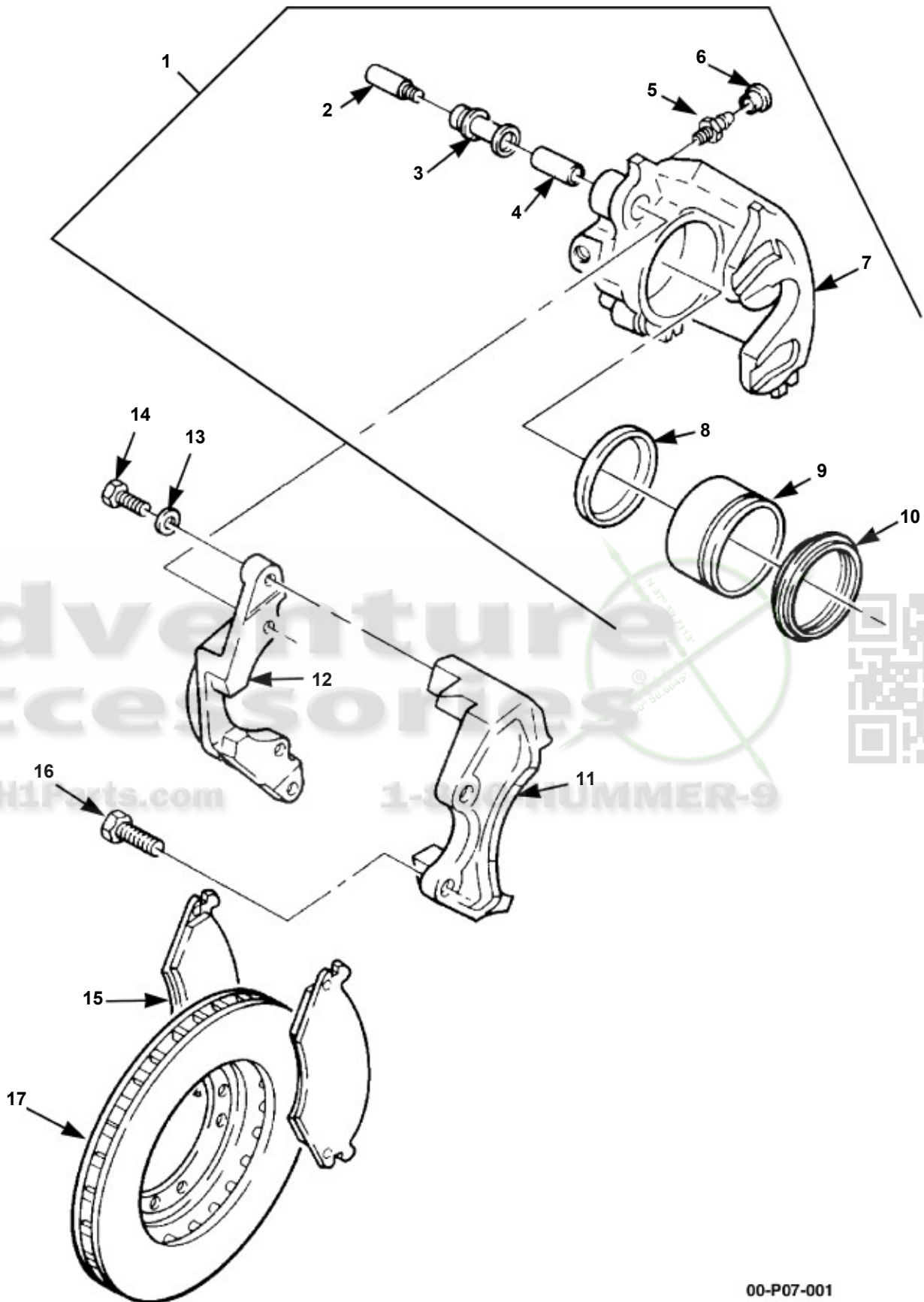
Front Service and Parking Brake Caliper Assembly and Rotor
