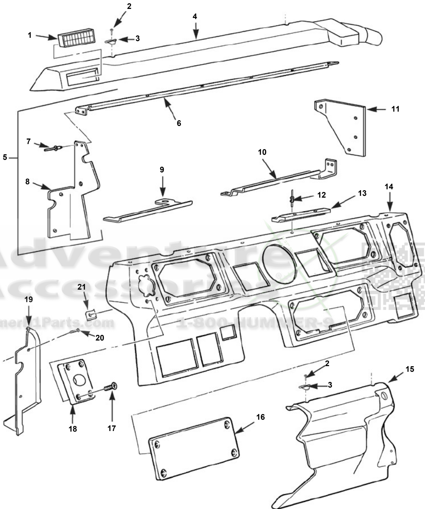
Instrument Panel Assembly, Dash Trim, Crash Pad, and Mounting Hardware
