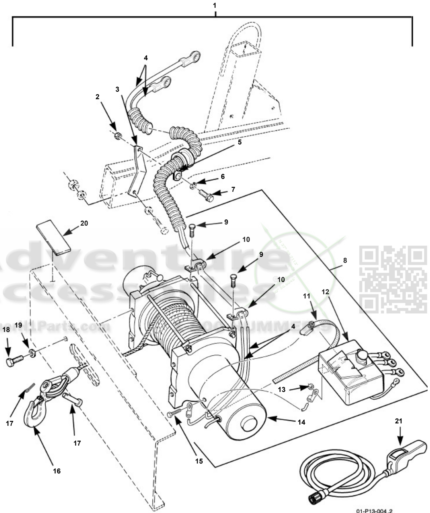
Winch Assembly, Mounting Hardware, and Related Parts (Winch Kit)
