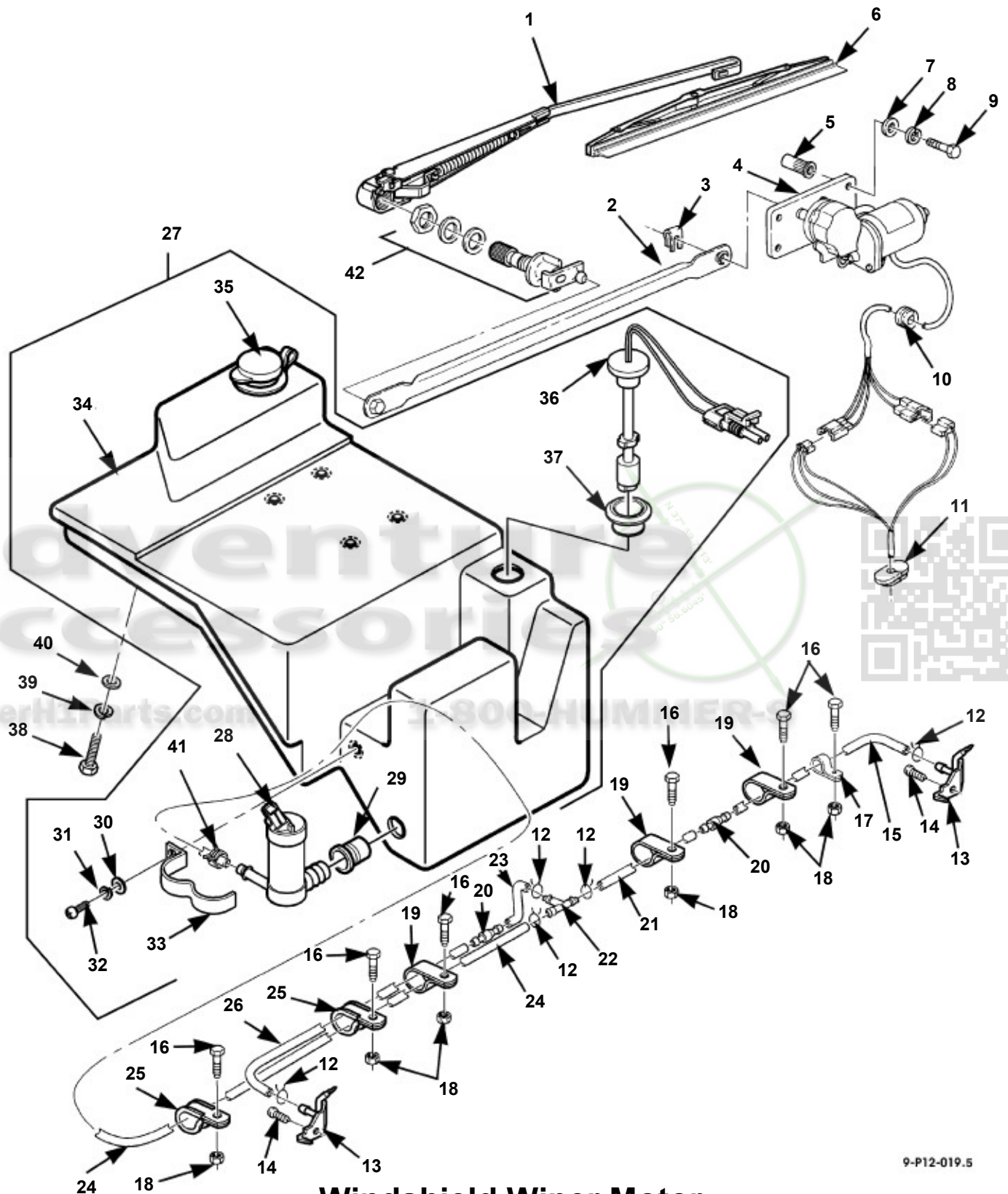
Windshield Wiper Motor, Wiper Assembly, and Washer Reservoir
