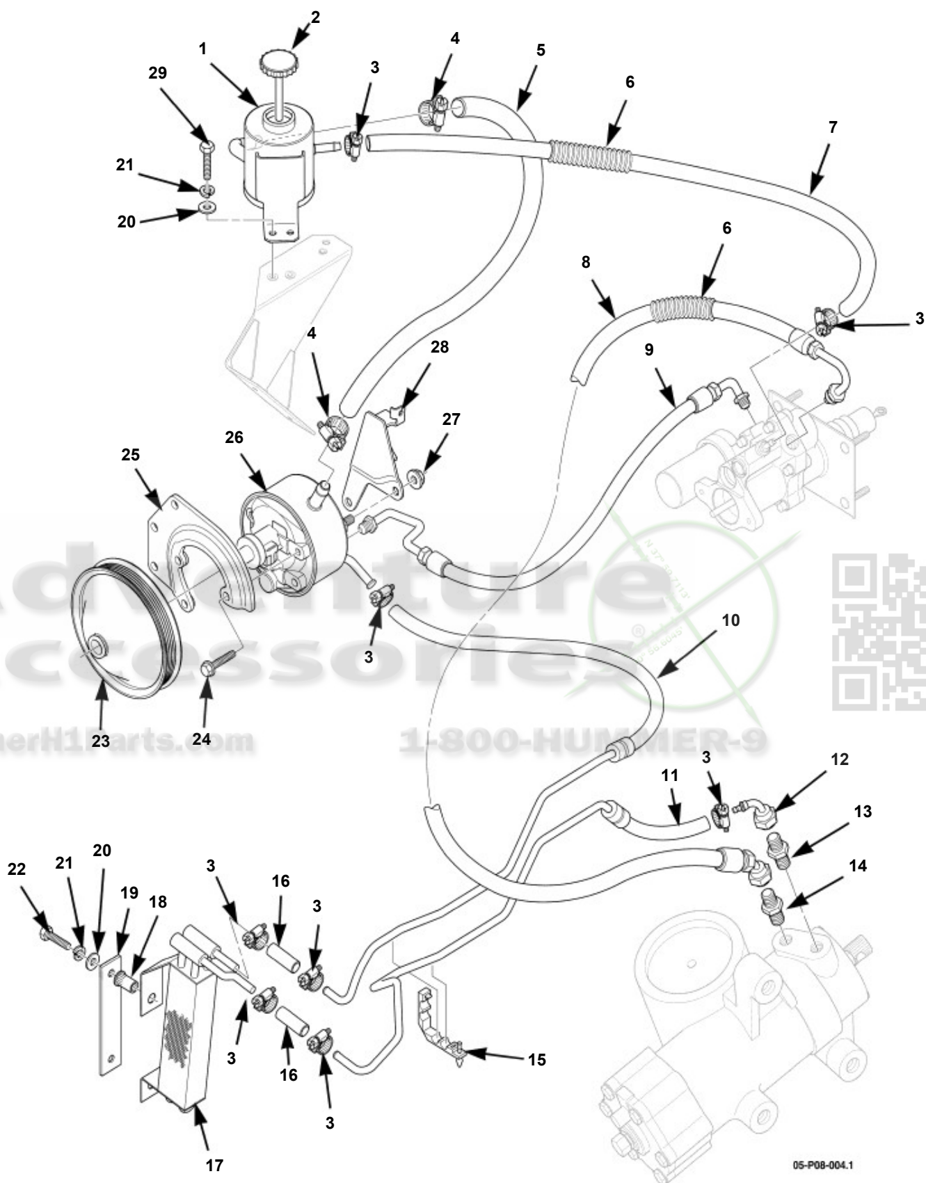
Power Steering Pump, Power Steering Reservoir, Oil Cooler Assembly, Pulley, Hoses, and Mounting Hardware
