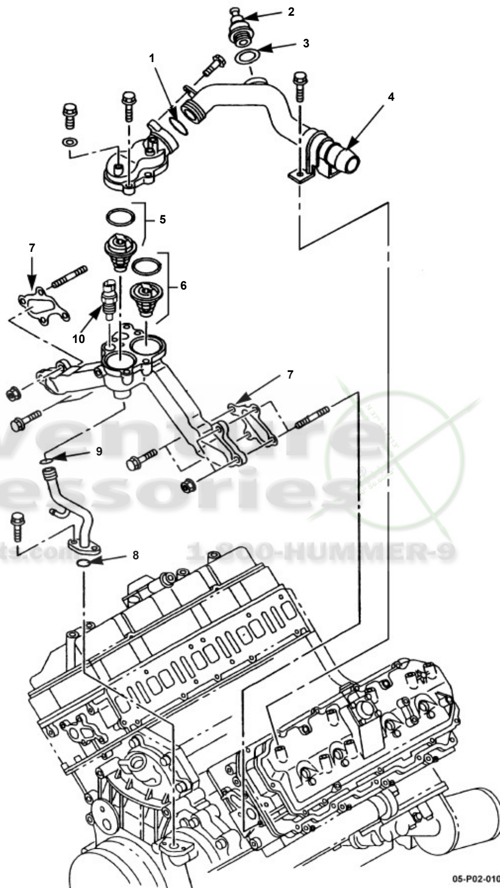
Thermostat, Water Crossover Gaskets, Thermal Coolant Valve and ECT Sensor
