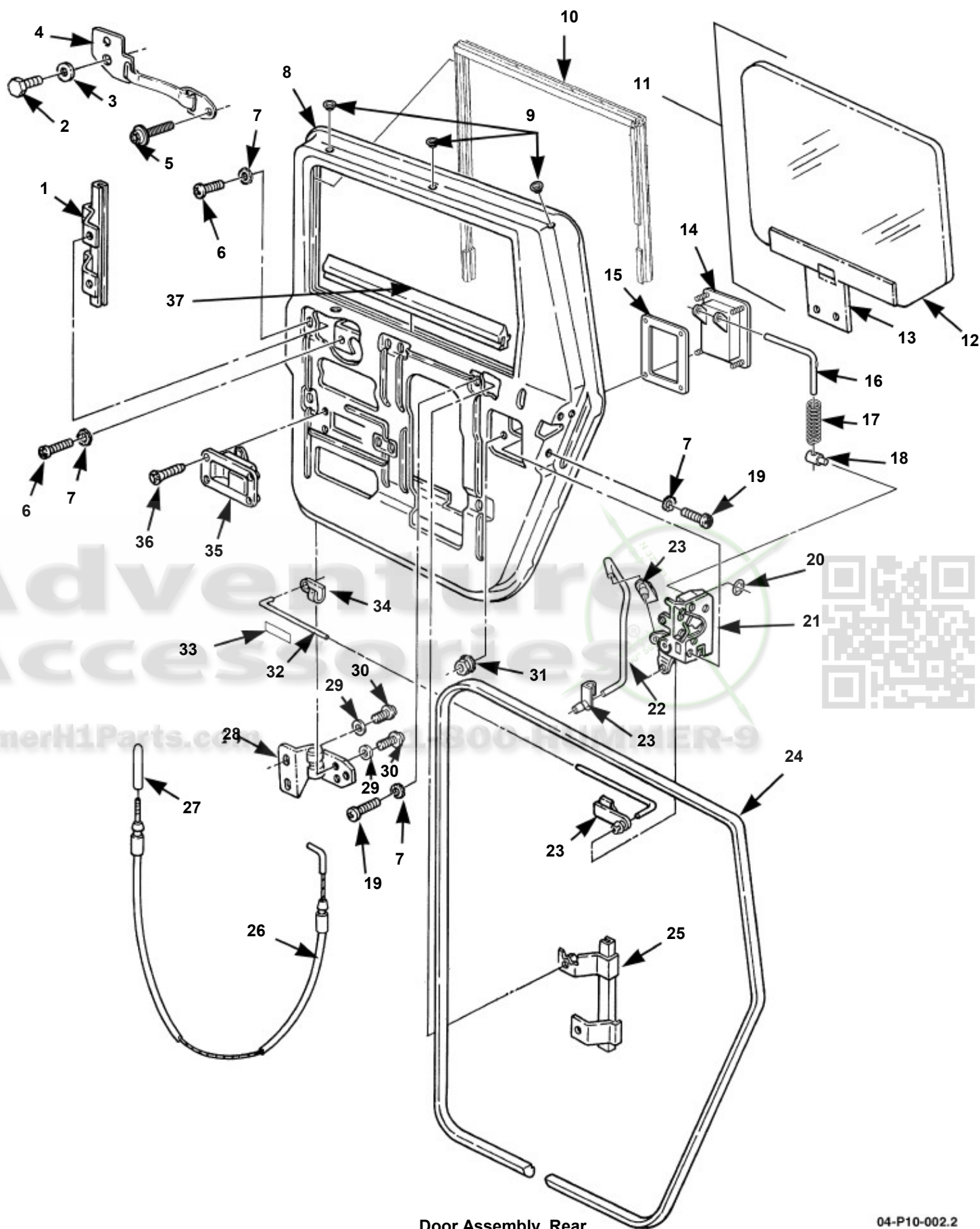
Door Assembly, Rear.
