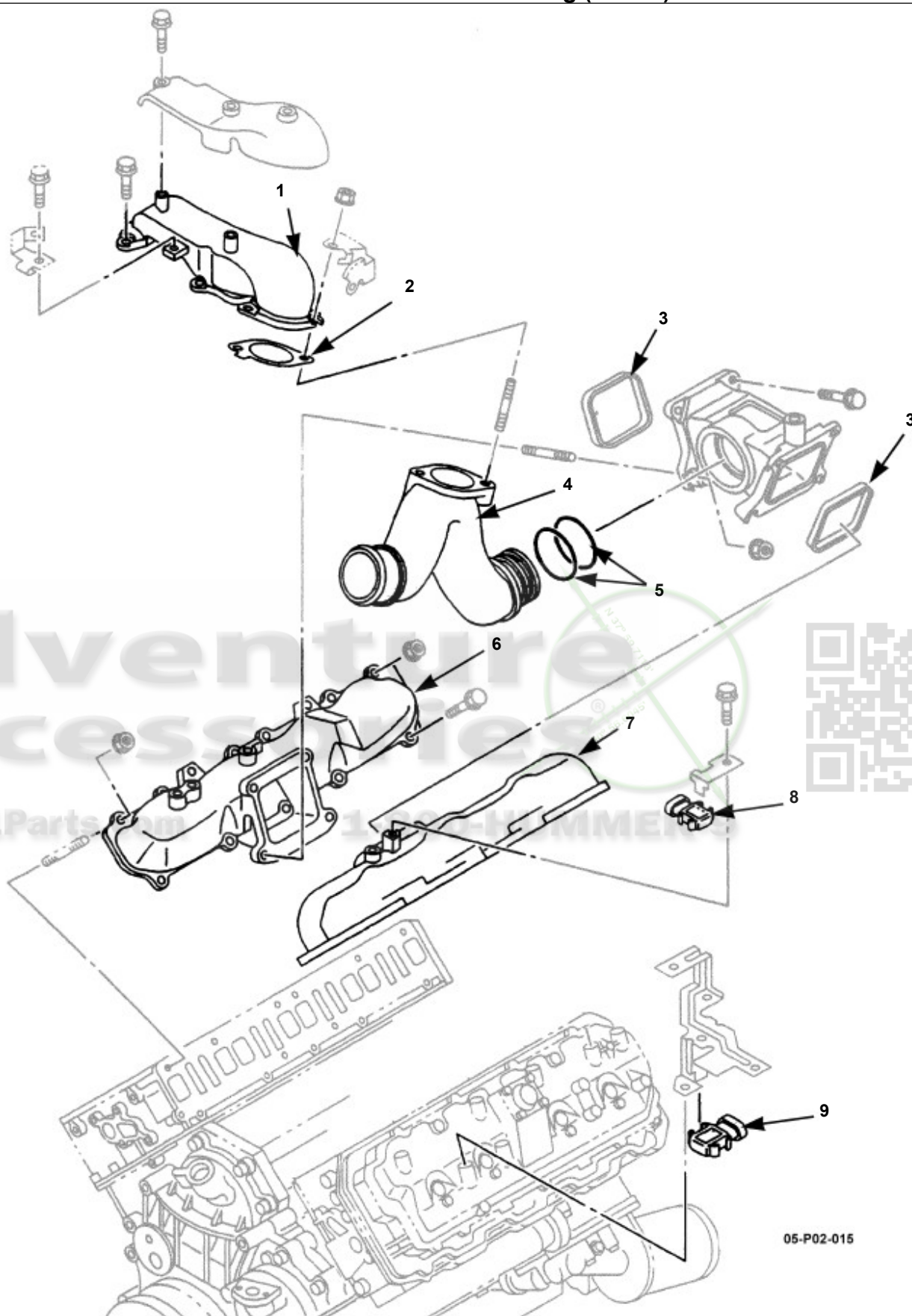
Inlet manifold, gaskets, Boost Sensor and Atmospheric Barometer Sensor
