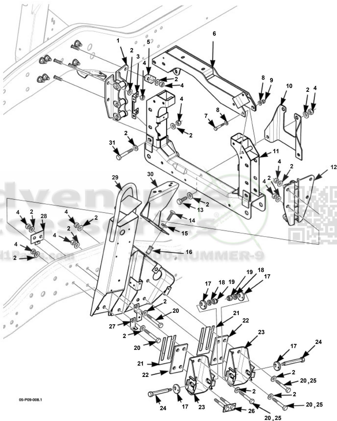
Front Suspension Crossmembers, Related Parts and Mounting Hardware
