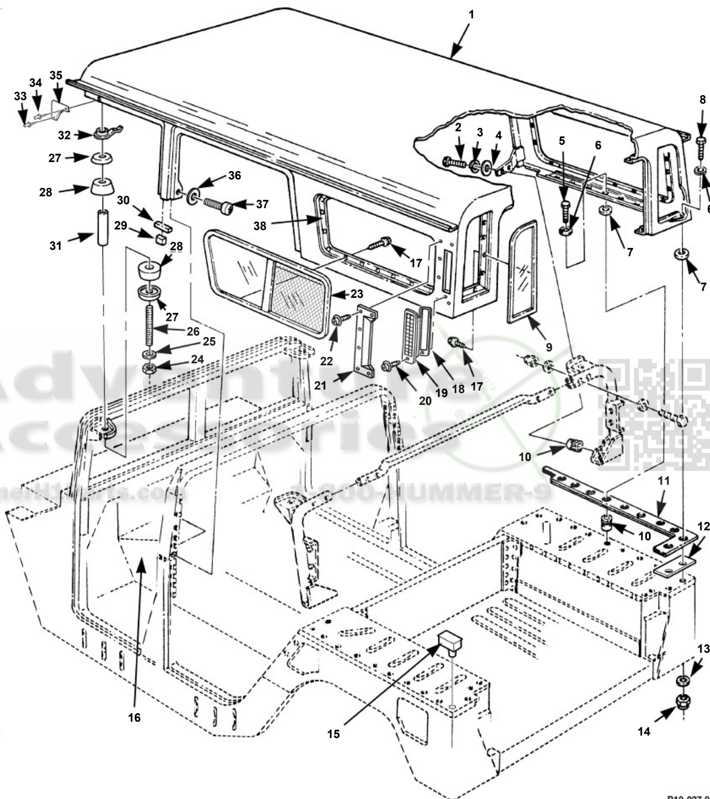
Roof and Mounting Hardware, Station Wagon, Model 84.
