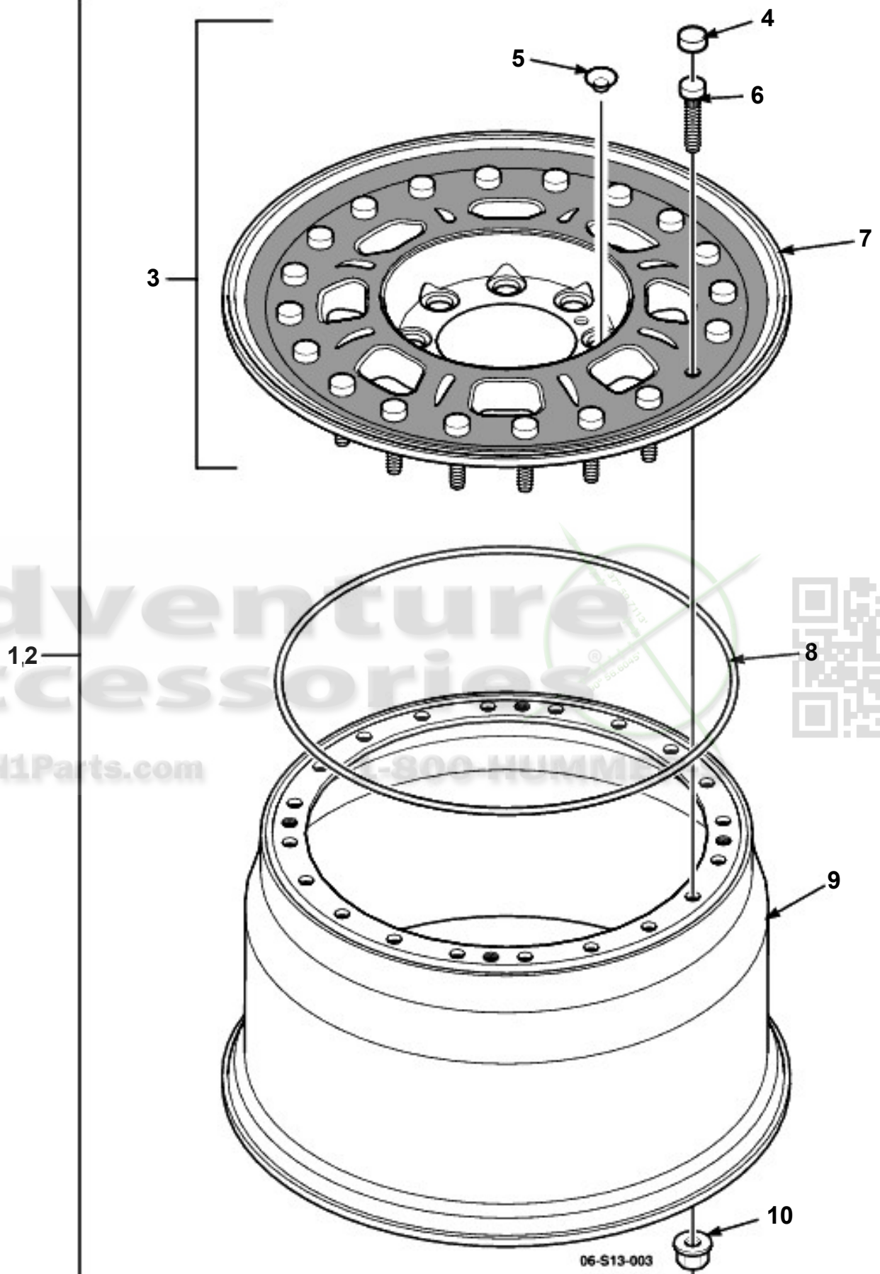
Wheel Assy, 17" 2-piece Aluminum w/Machined Windows, D
