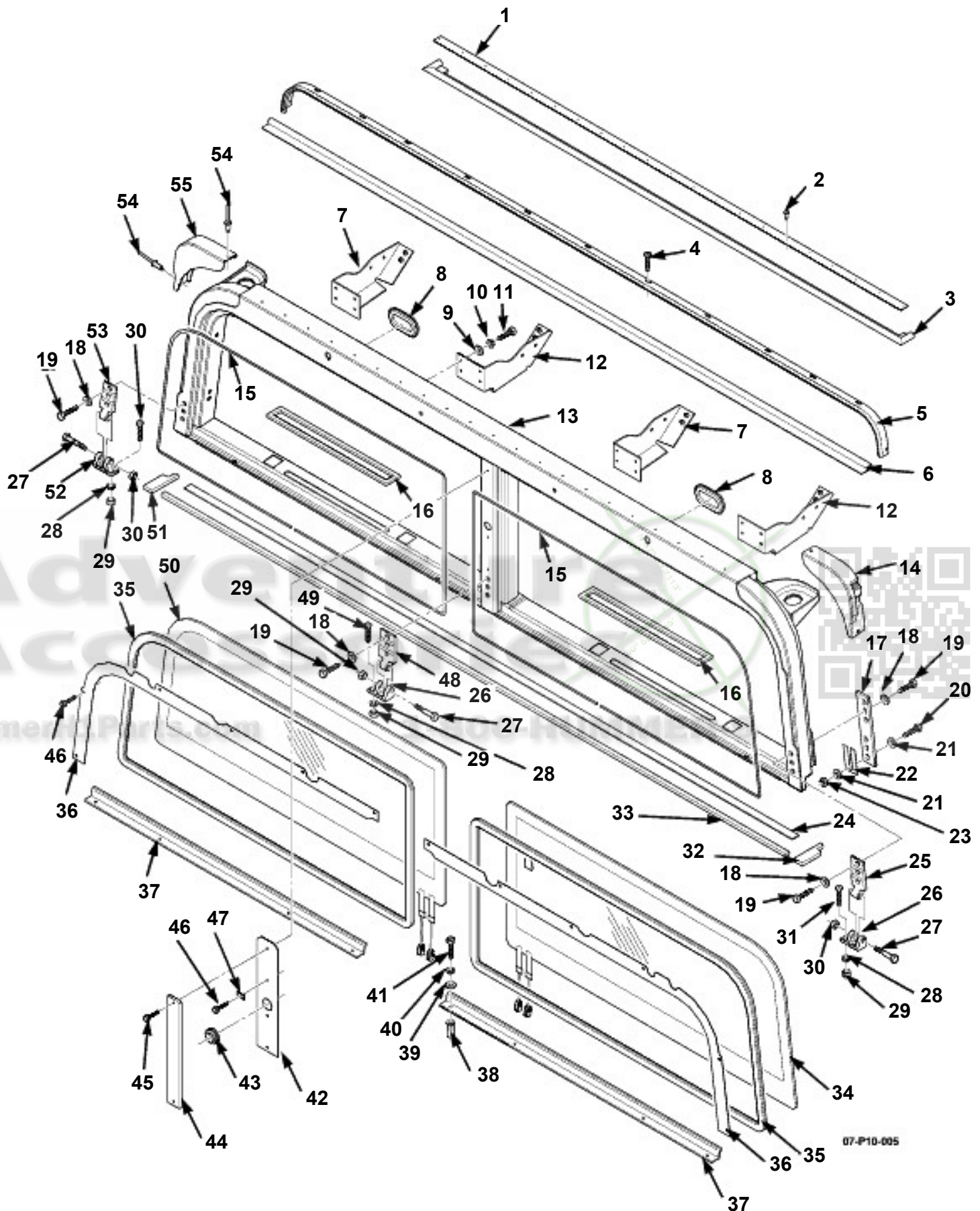
Windshield Assembly.
