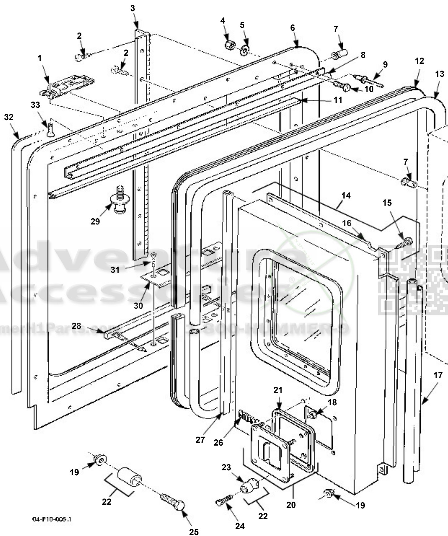
Station Wagon Vertical Doors, Model 84. (Sheet 1 of 2)
