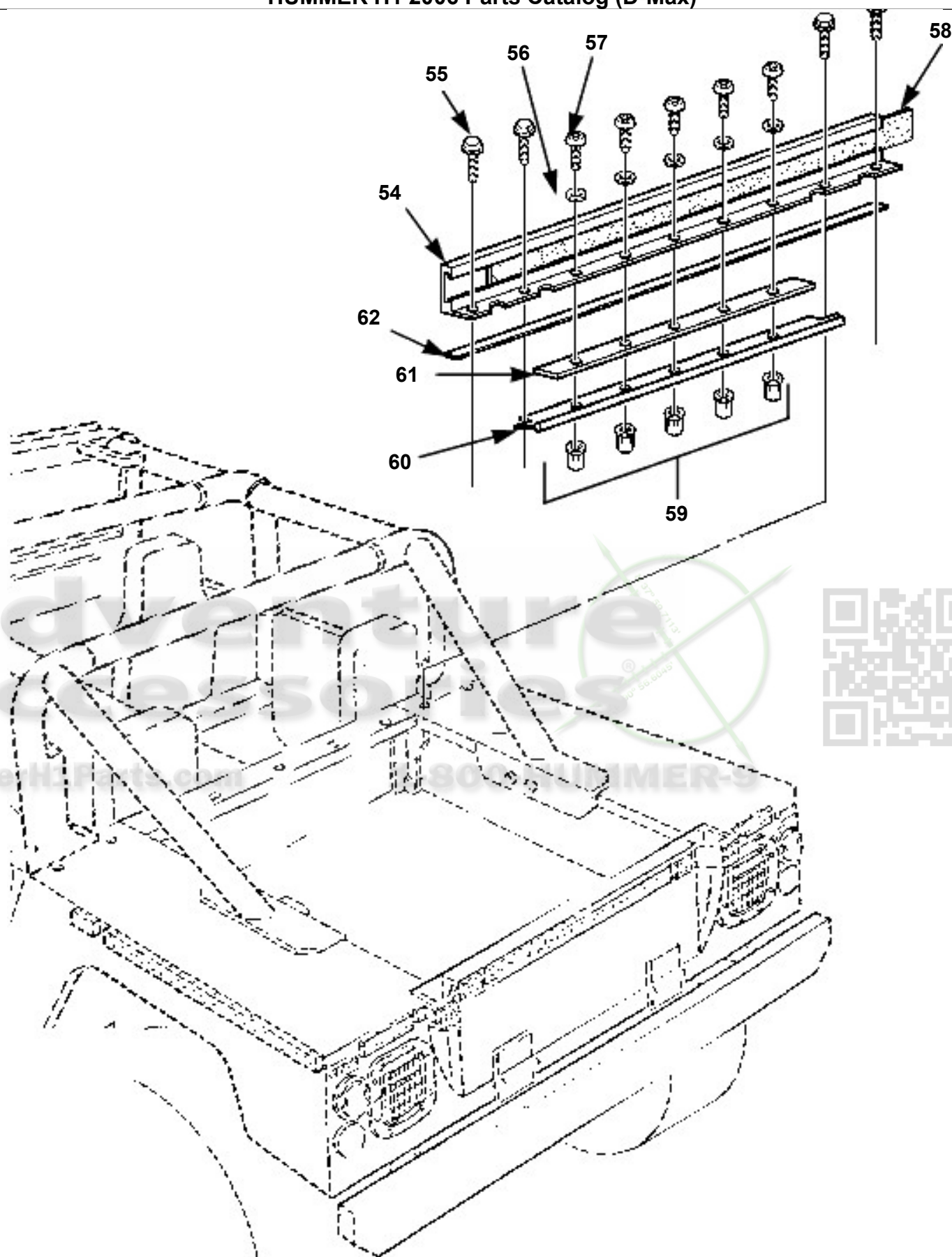
Soft Top Support Structure, Support Bar, Model 90. (Sheet 2 of 2)
