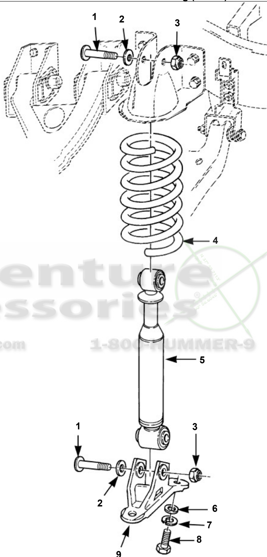
Shock Absorbers and Springs, Front and Rear
