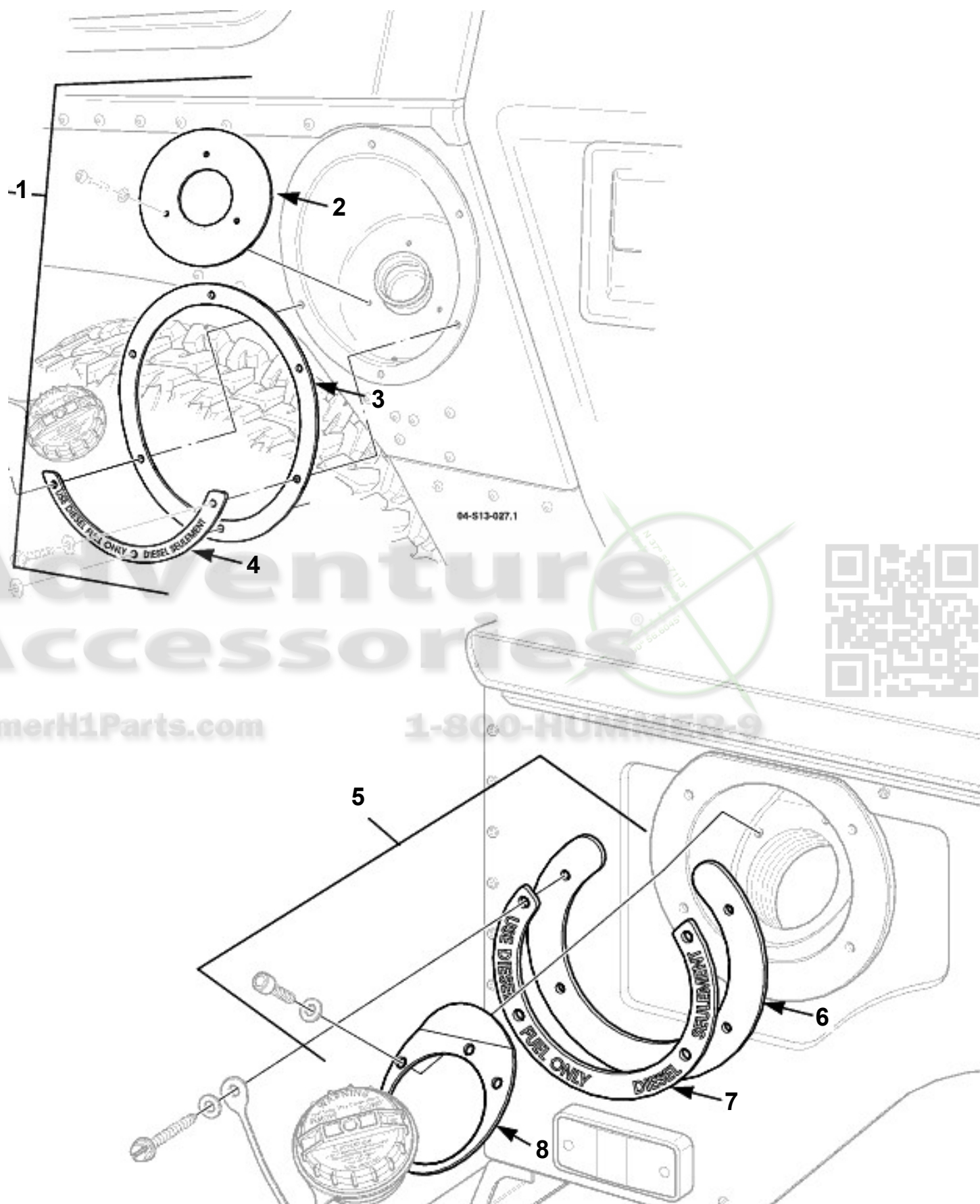
Fuel Tank Filler Applique, Main and Auxiliary, Stainless Steel
