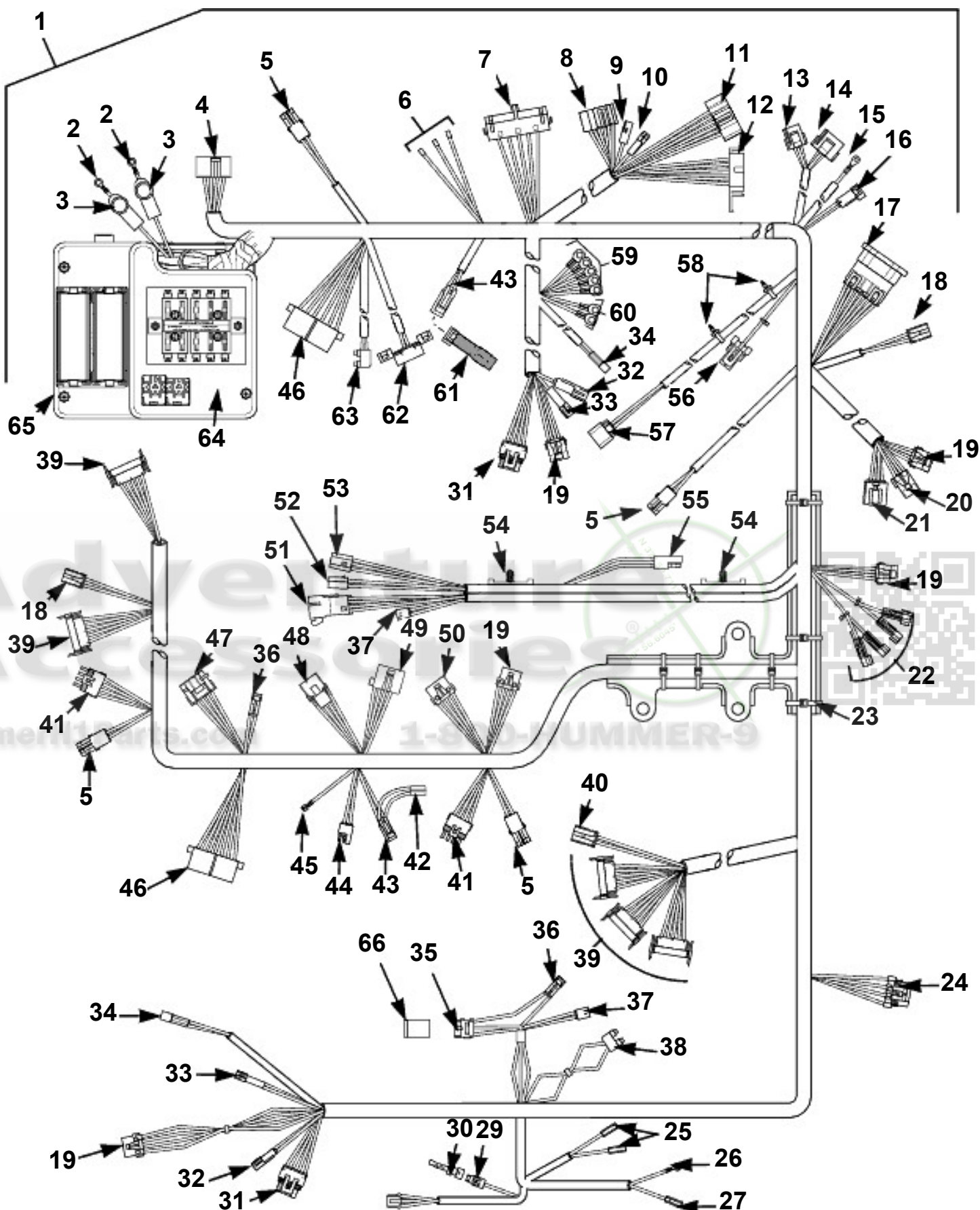
Harness Assembly, Cross Body (1 of 3)
