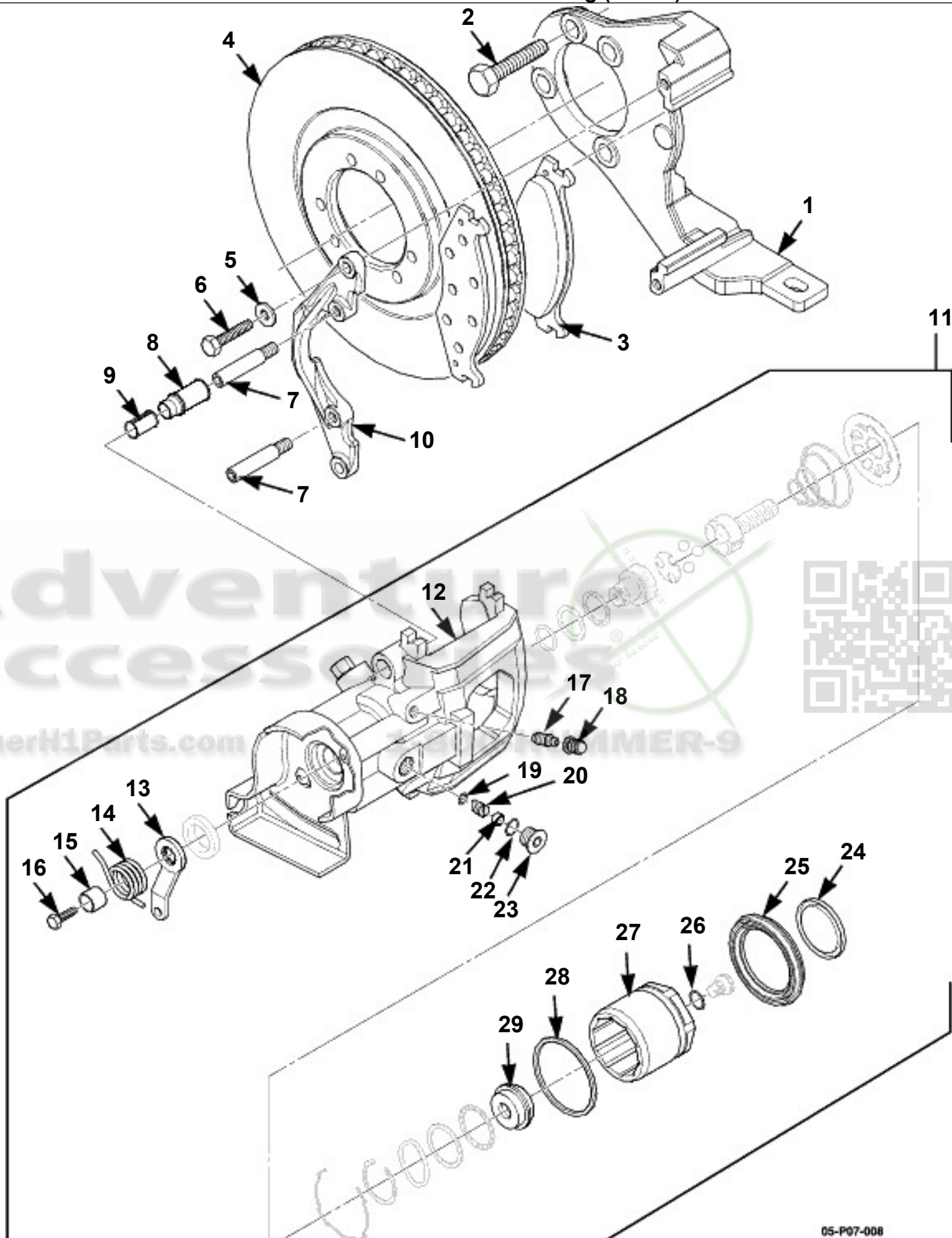
Rear Service and Parking Brake Caliper Assembly and Rotor
