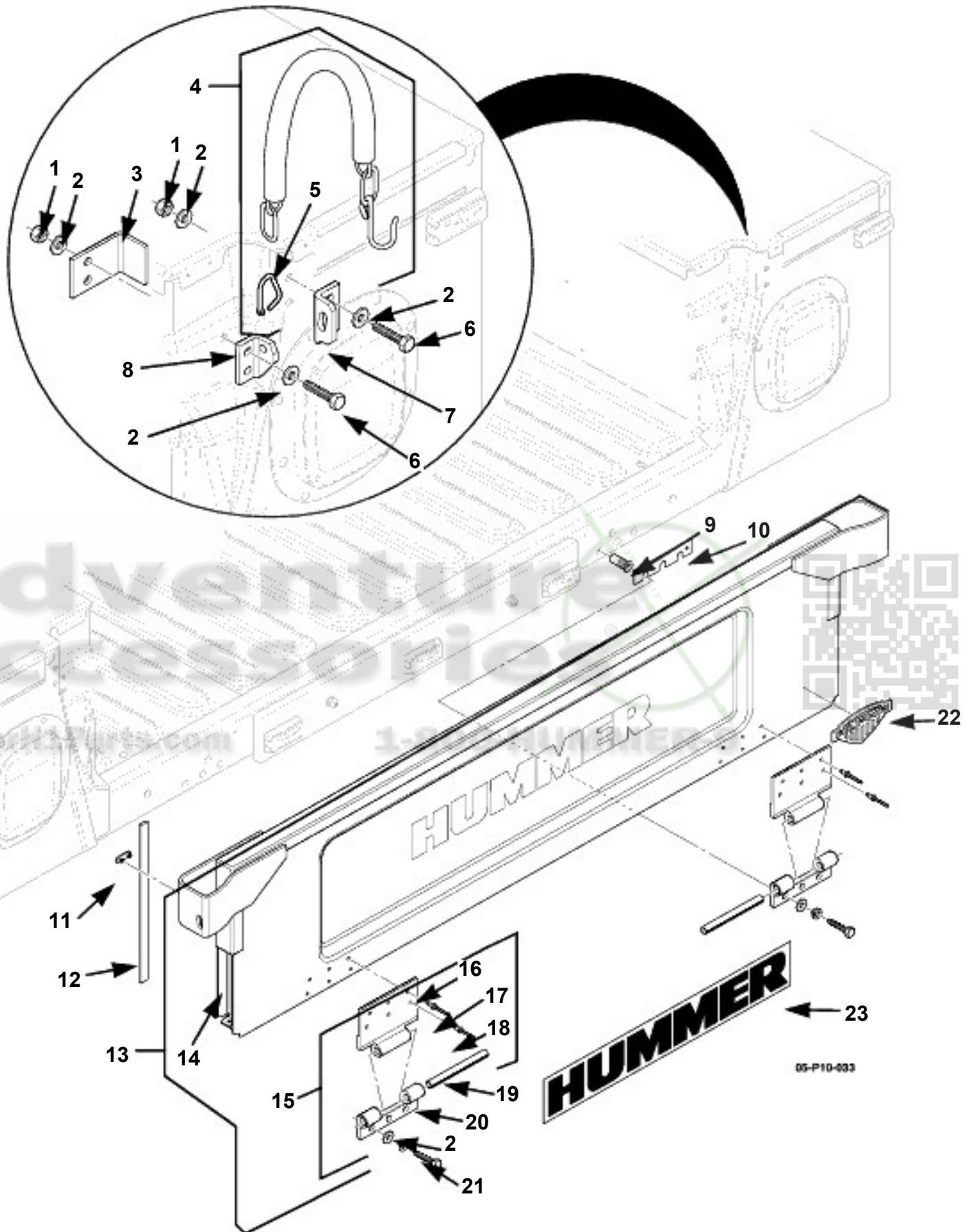
Tailgate Assembly and Related Parts.
