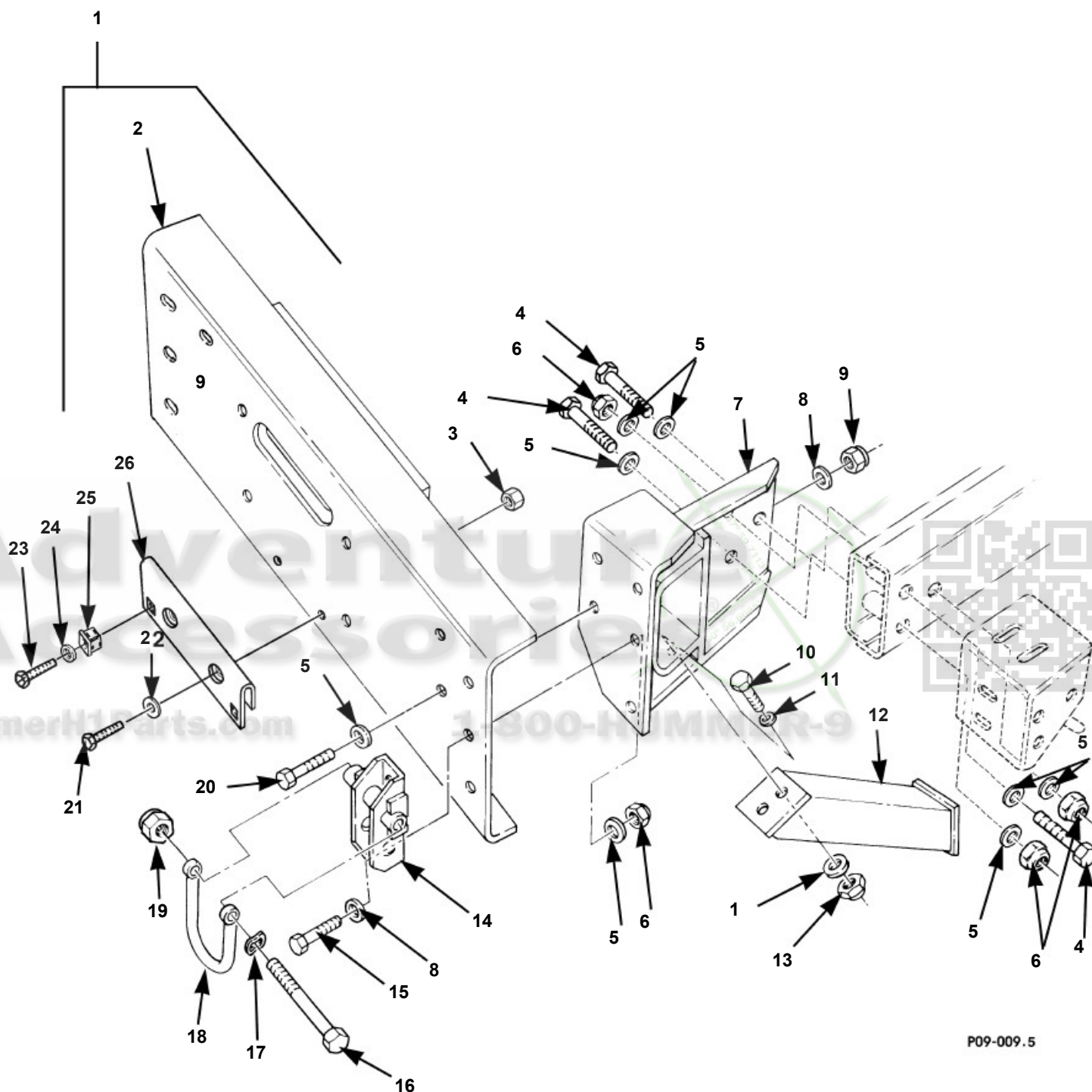
Winch Bumper, Winch Assembly, Mounting Hardware and Related Parts (Winch Kit) Graphic 1 of 2
