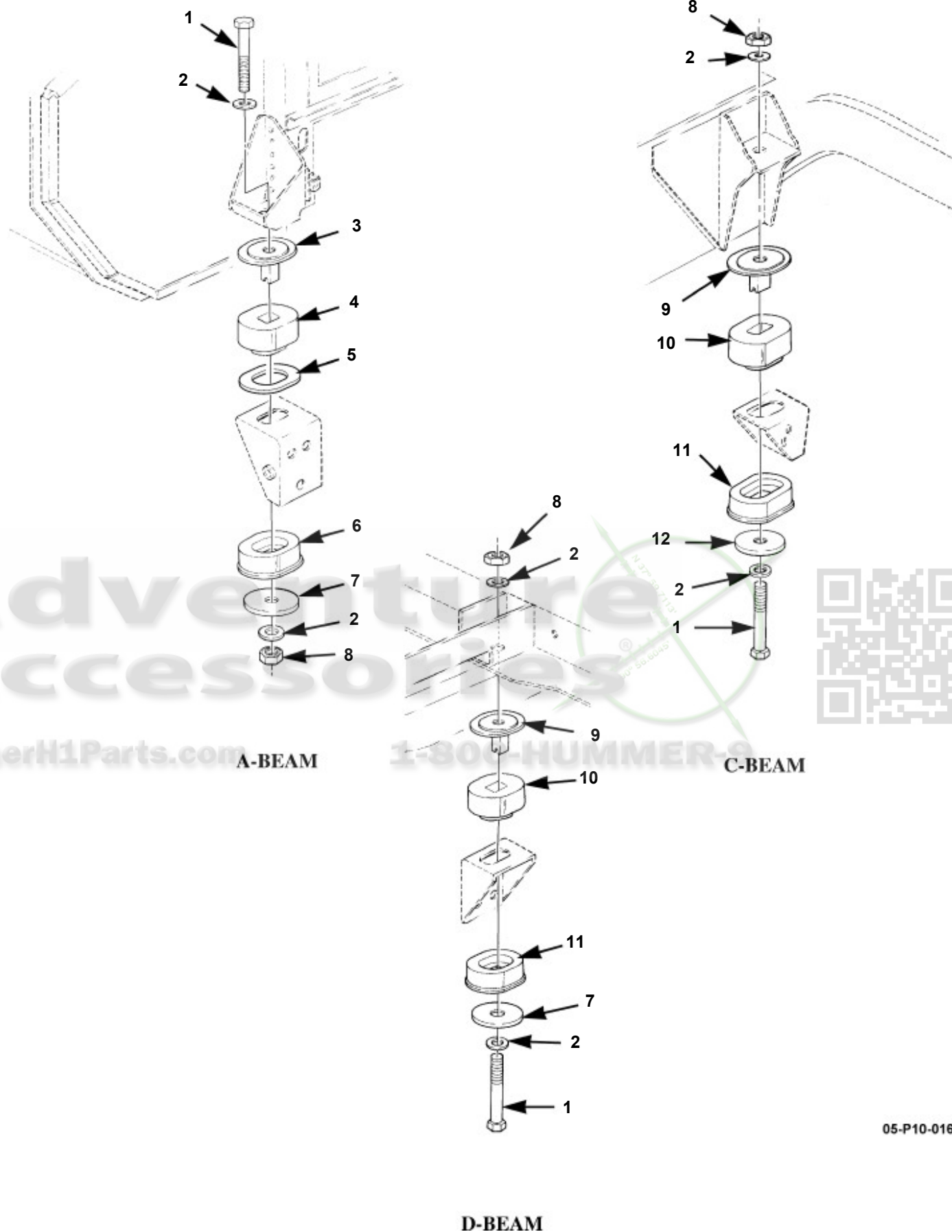
Body Mounting Components, "A", "C", and "D" - Beams.
