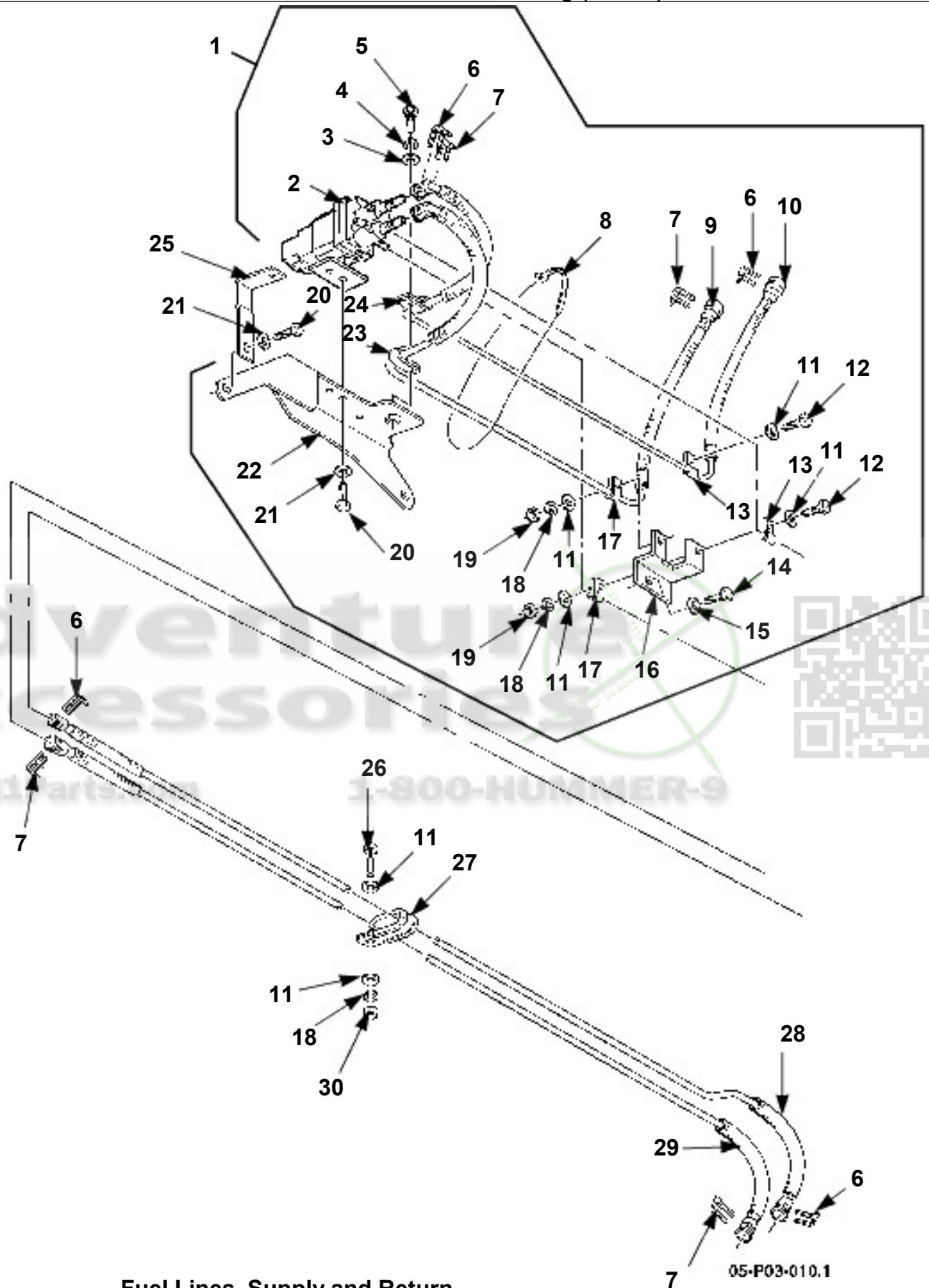
Fuel Lines, Supply and Return, Tank Selector Switch to Tanks
