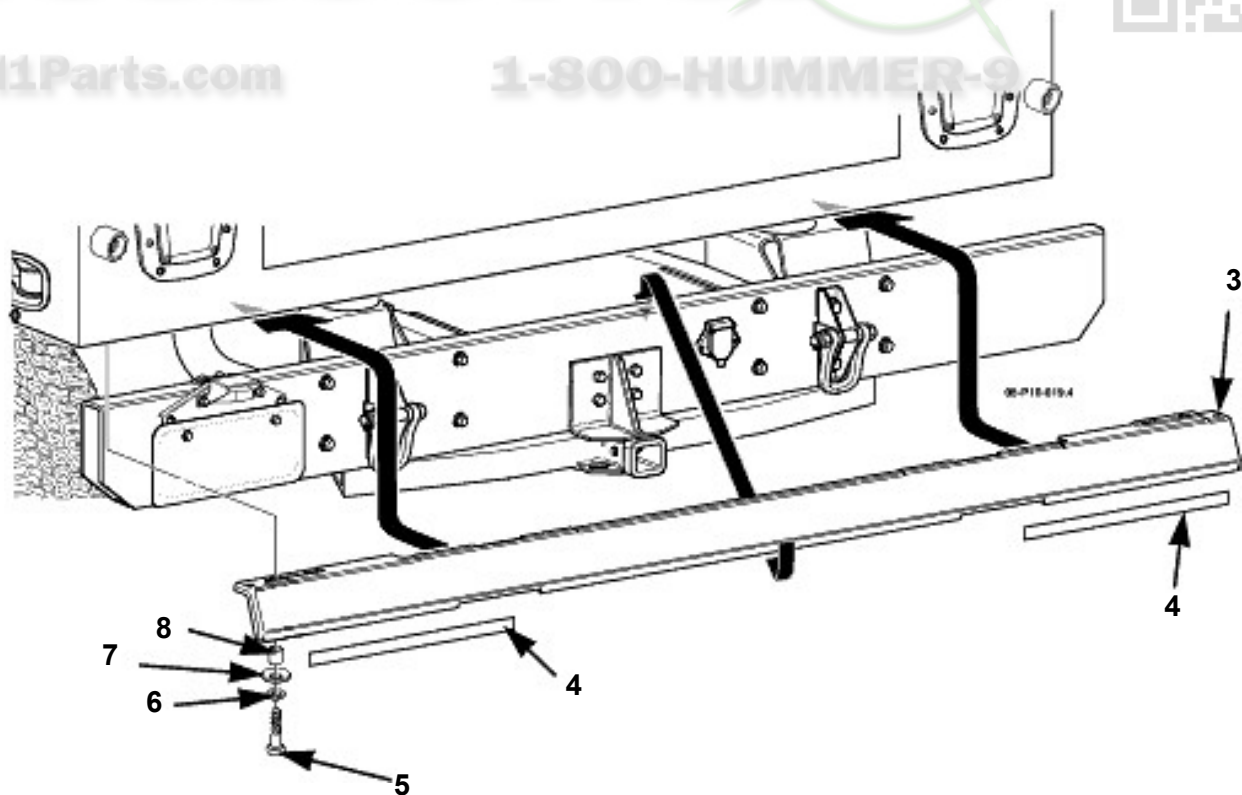
Wheel Well Closeout and Rear Closeout.
