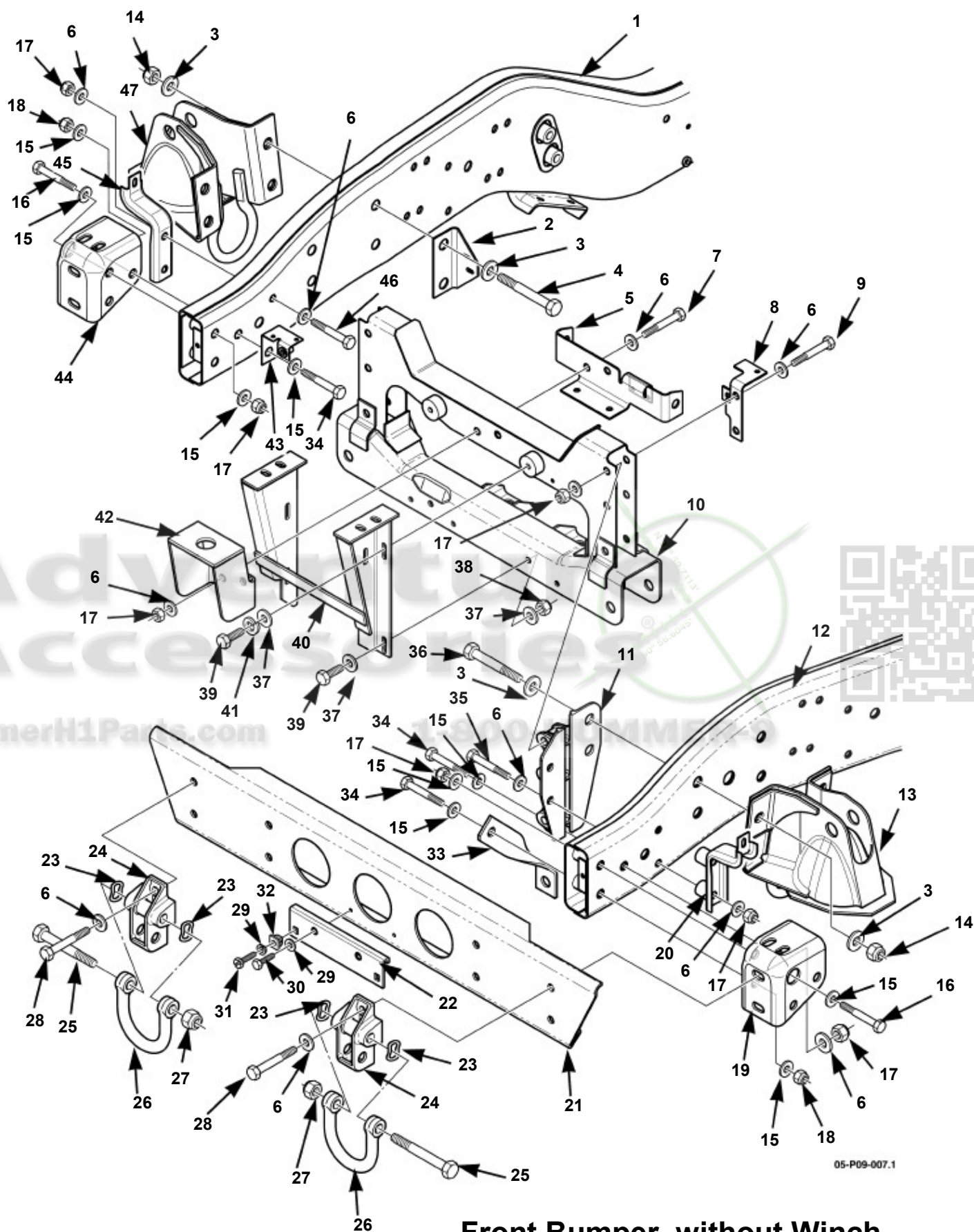
Front Bumper, without Winch
