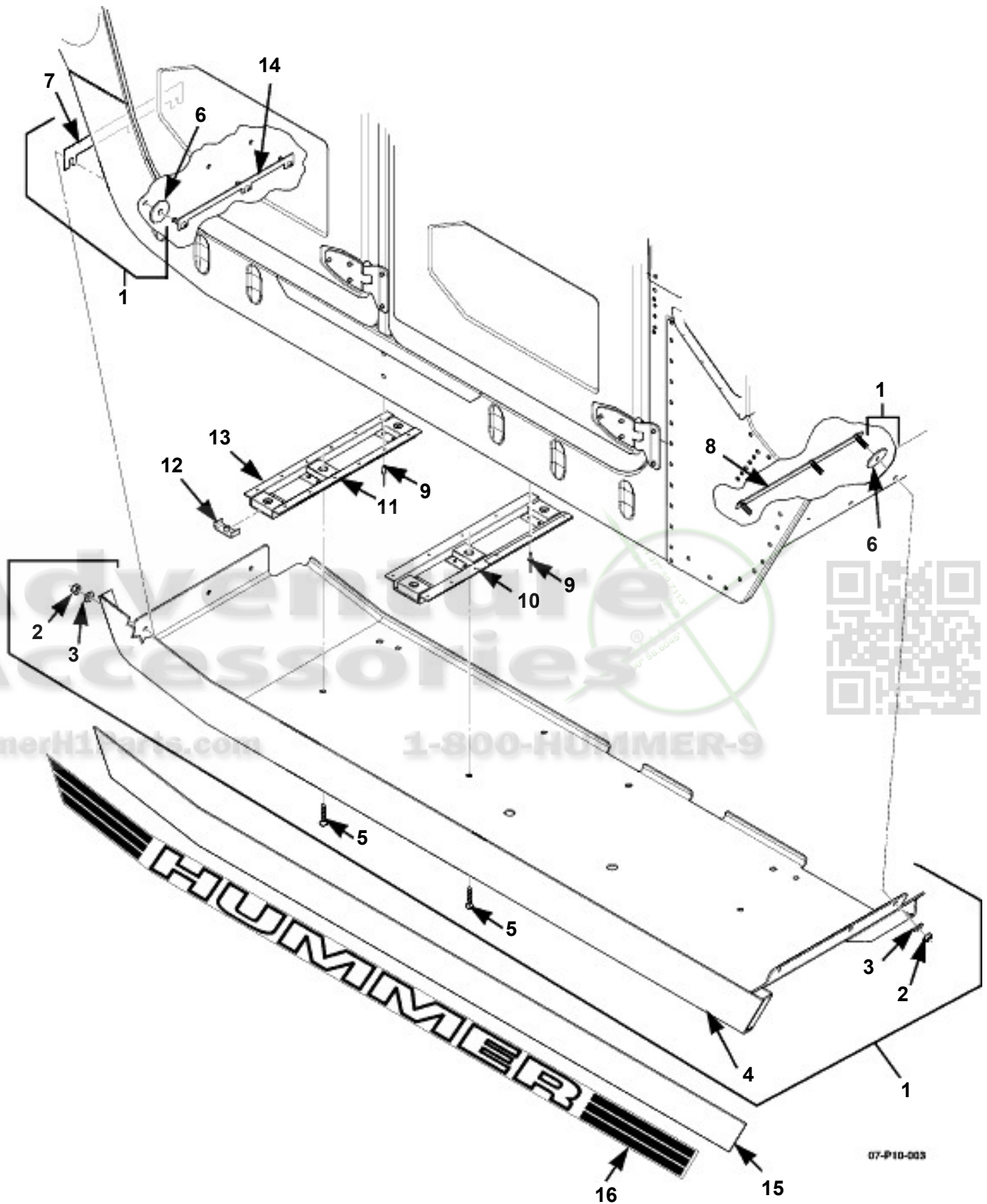
Rocker Panel Guard Protection.
