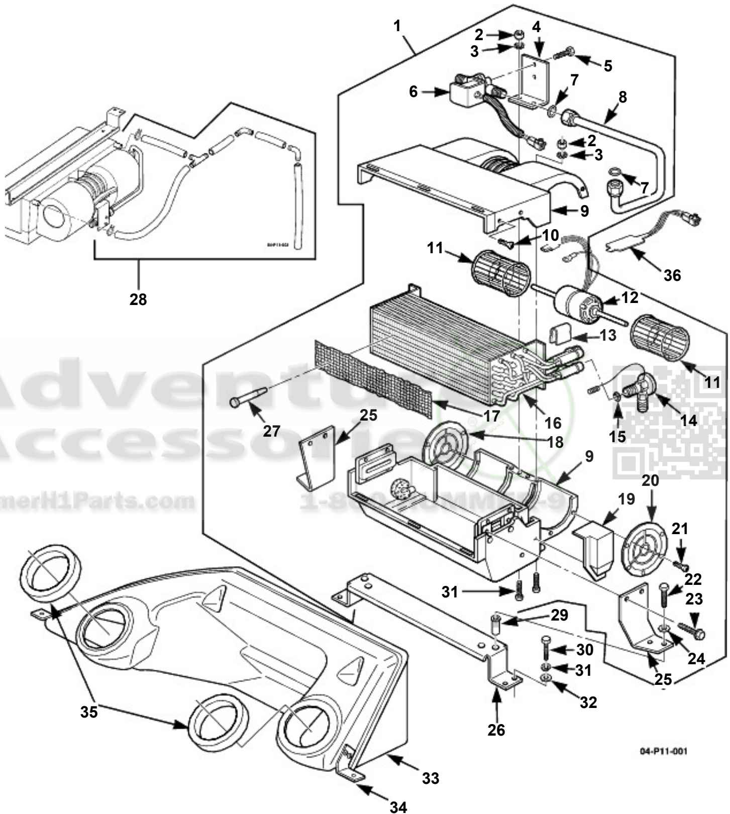
Auxiliary HVAC Unit
