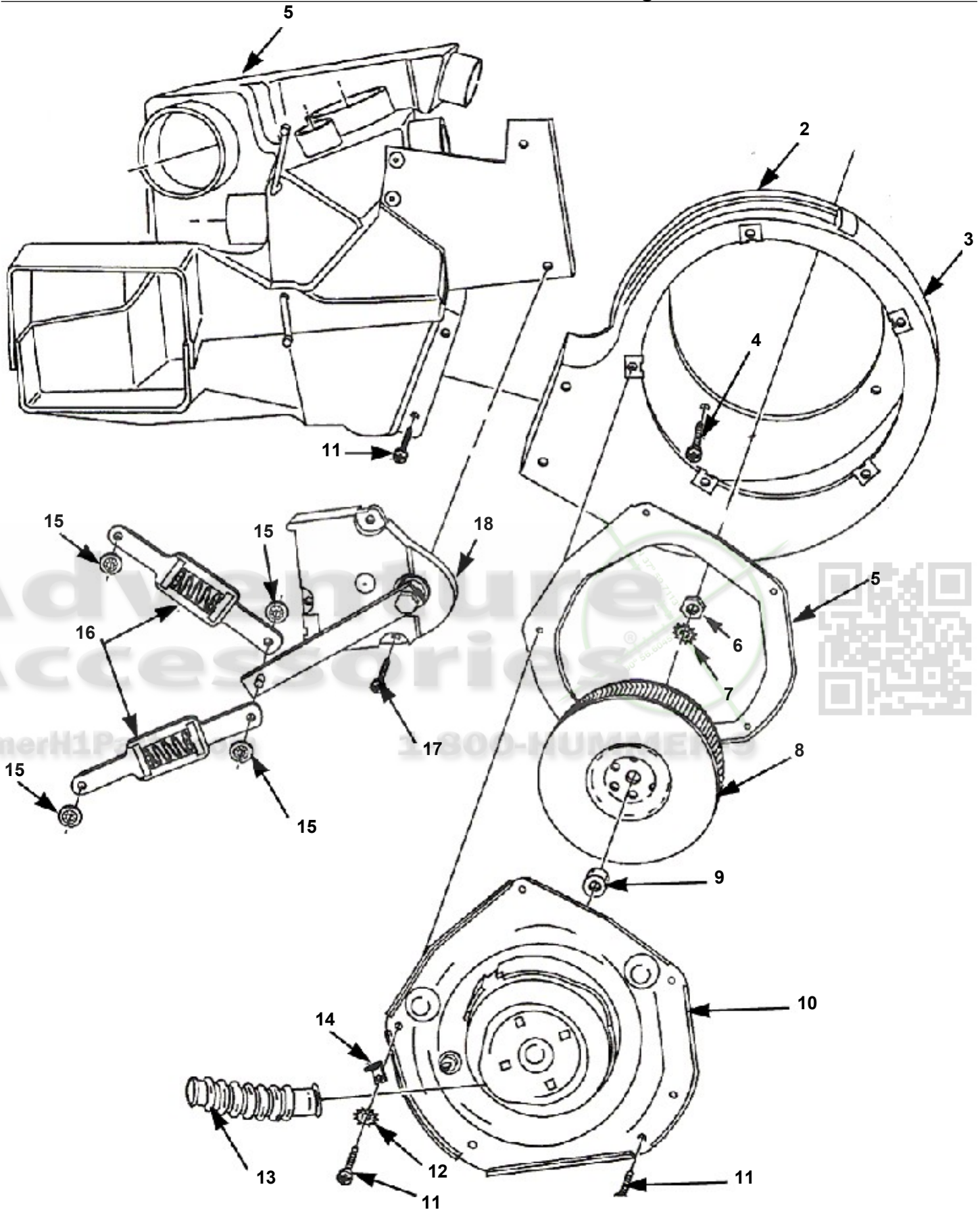
Diverter and Blower Motor Assembly
