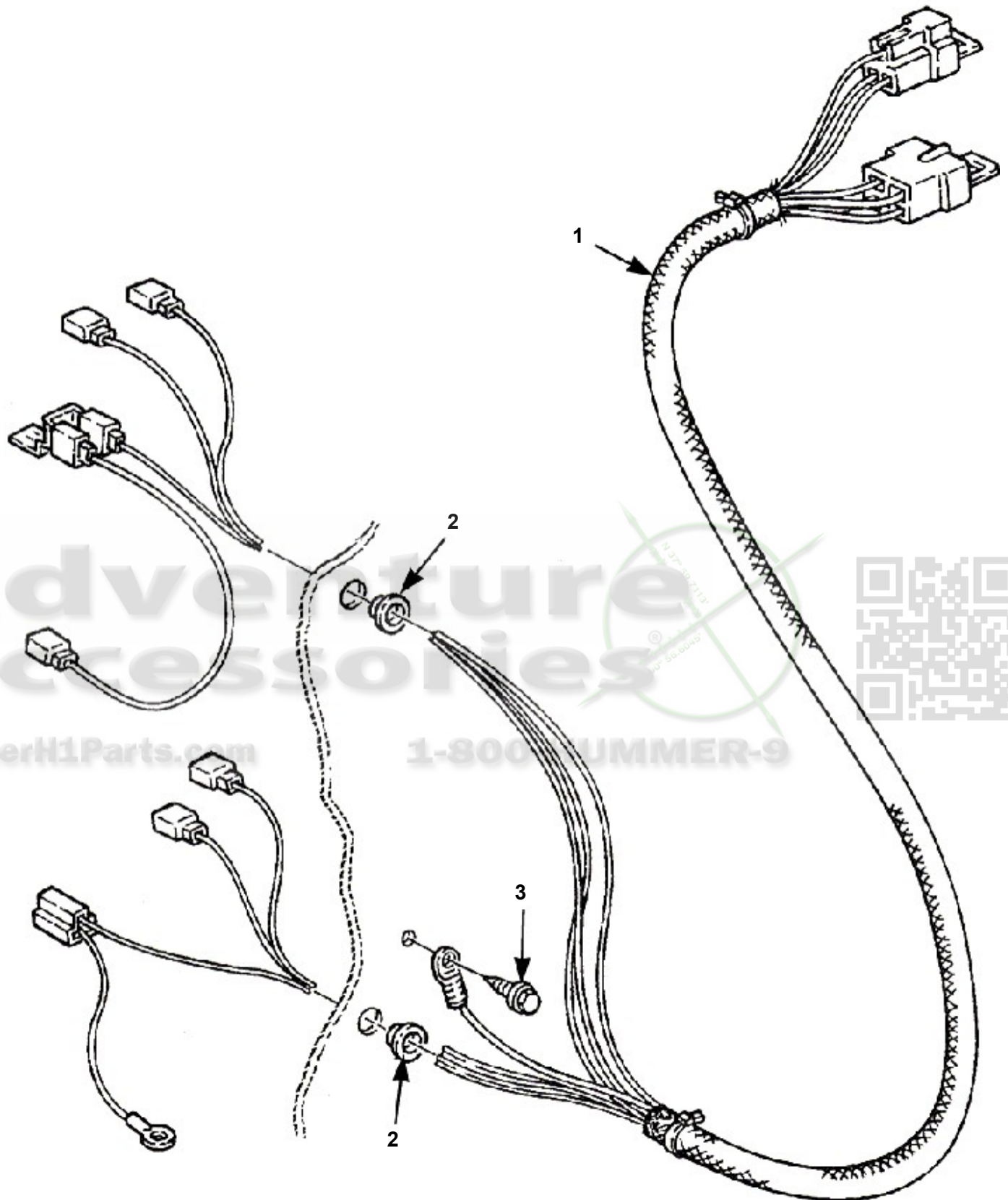
Harness Assembly, Main A/C -Heat (1992 and 1993 only)
