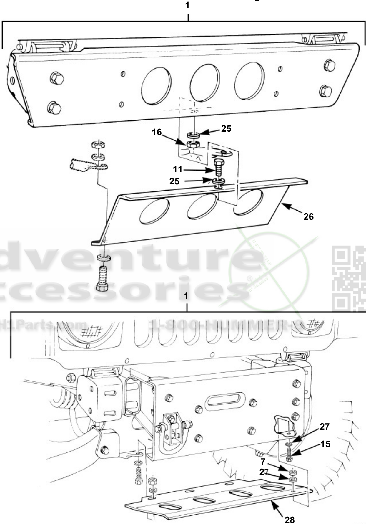
Underbody Protection and Mounting Hardware (Figure 2 of 2)
