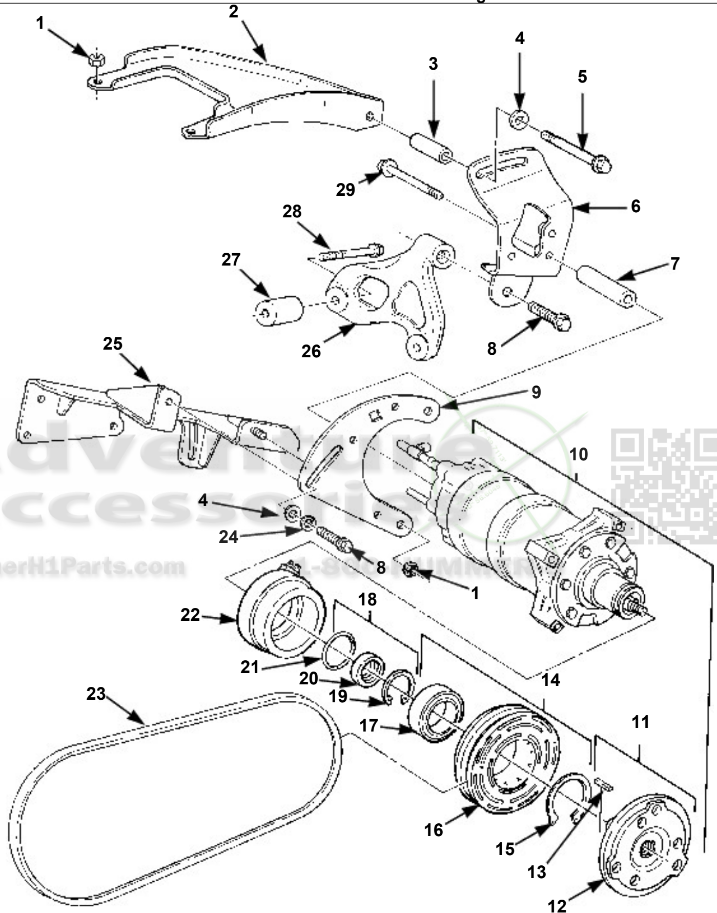
Air Conditioner Compressor and Mounting Hardware (1992 and 1993 only)
