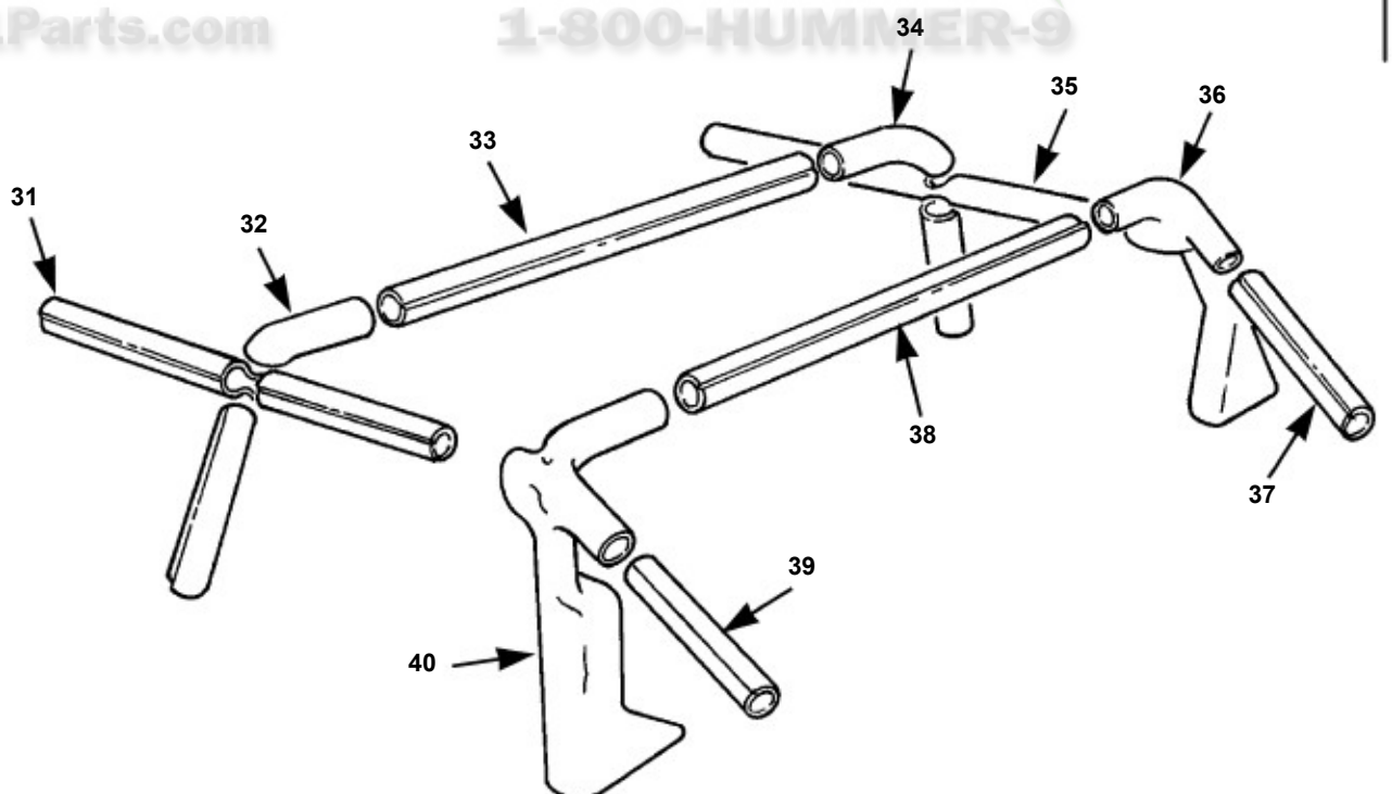
Soft Top Kit and Support Structure (Figure 1 of 2)
