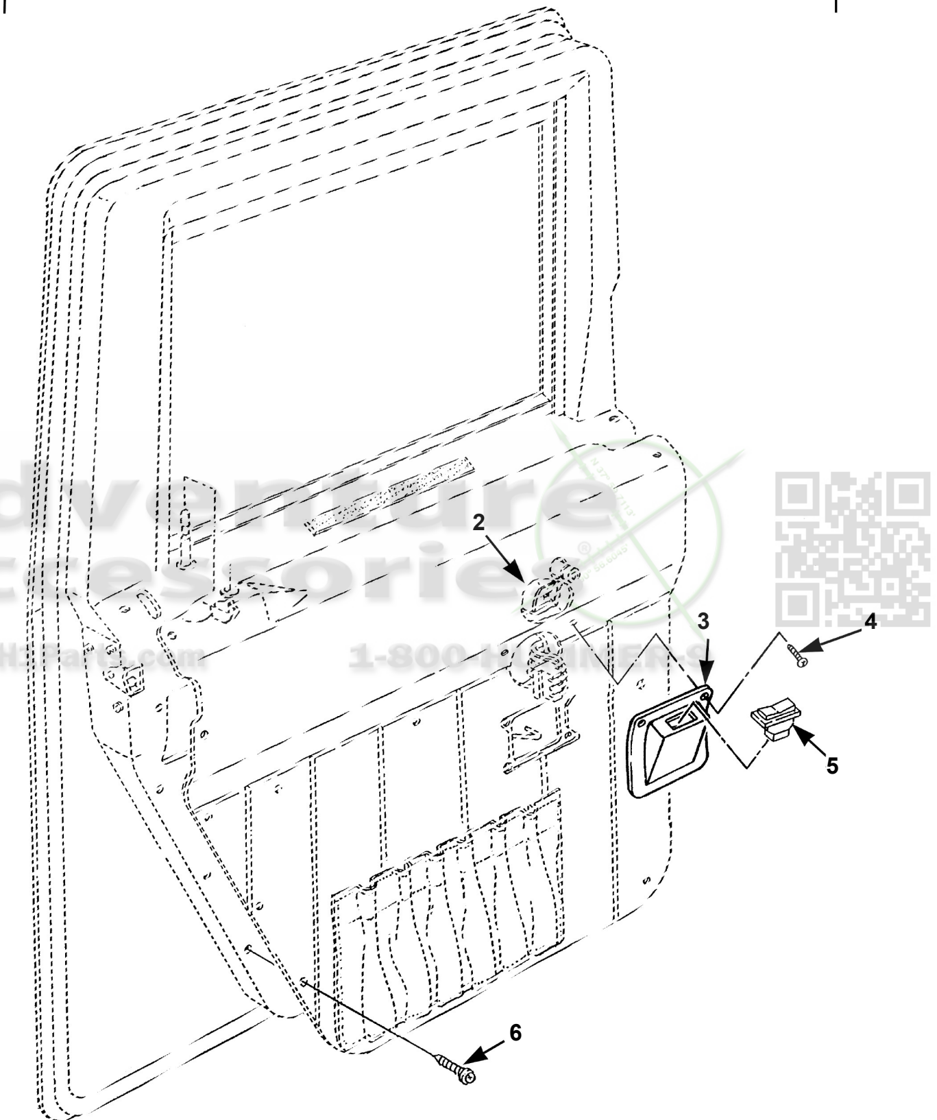
Two-Door and Four-Door Power Door Locks Kit (Graphic 1 of 8) P12-052
