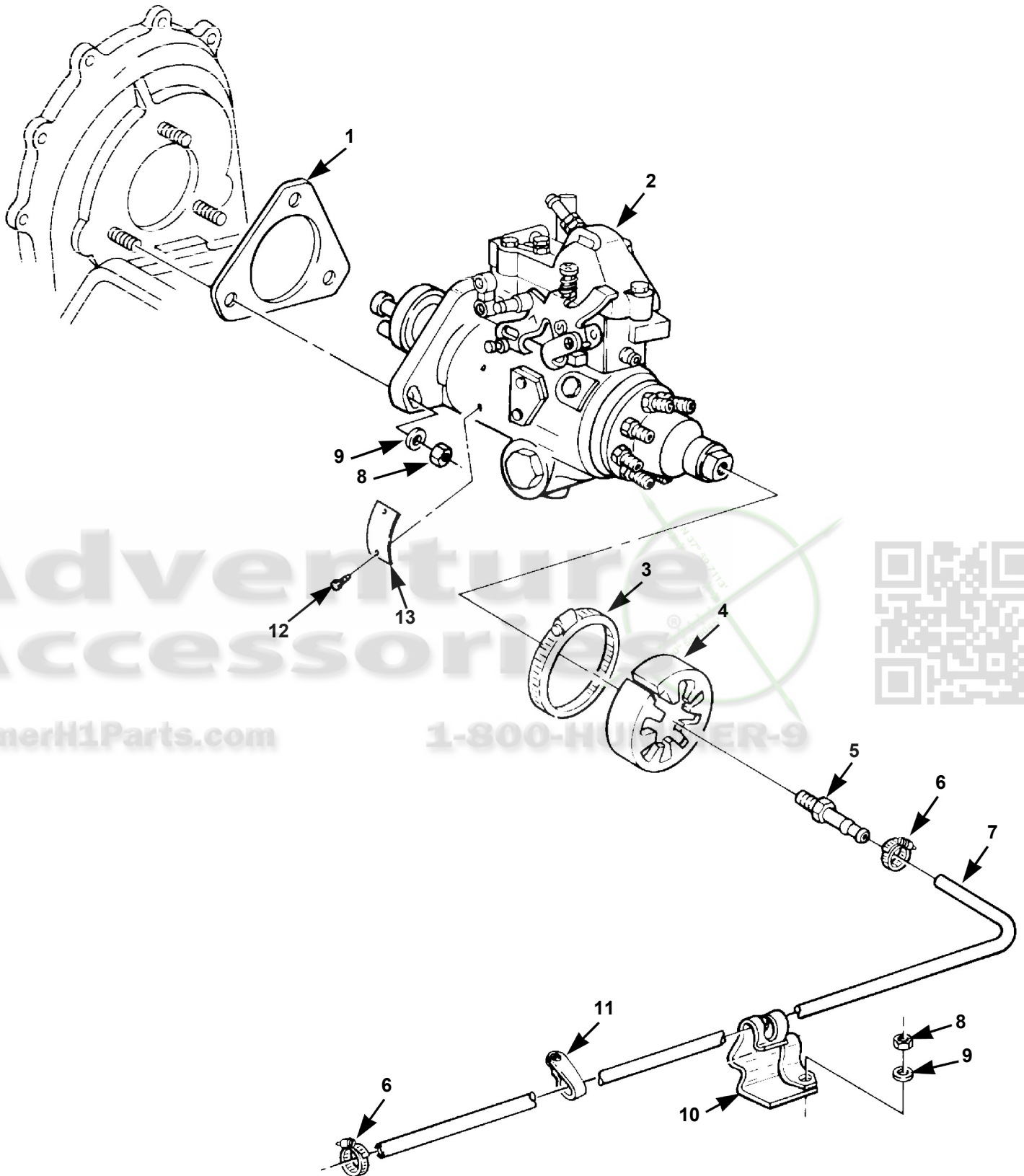
Fuel Injection Pump and Fuel Filter Lines.
