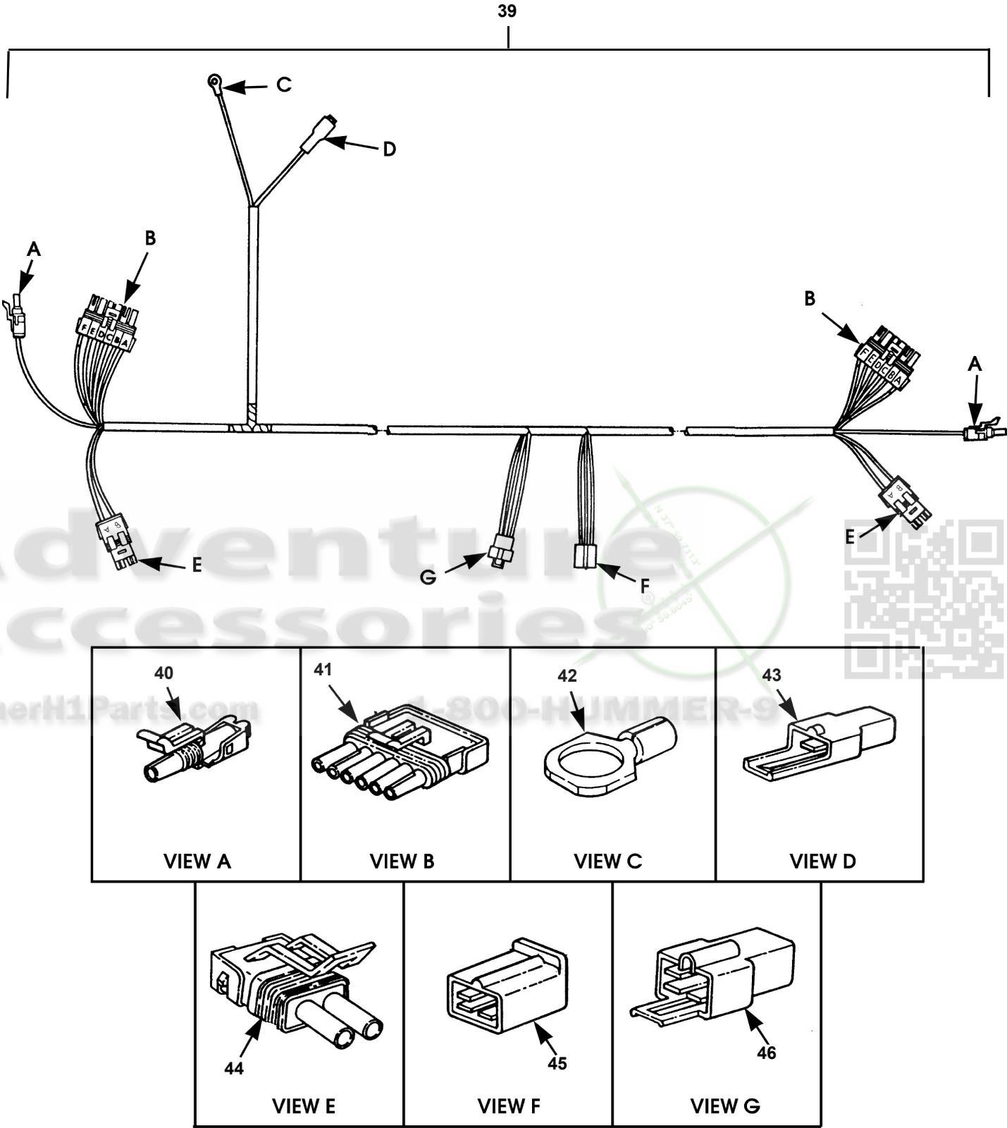
Two-Door and Four-Door Power Locks Kit (Graphic 7 of 8)
