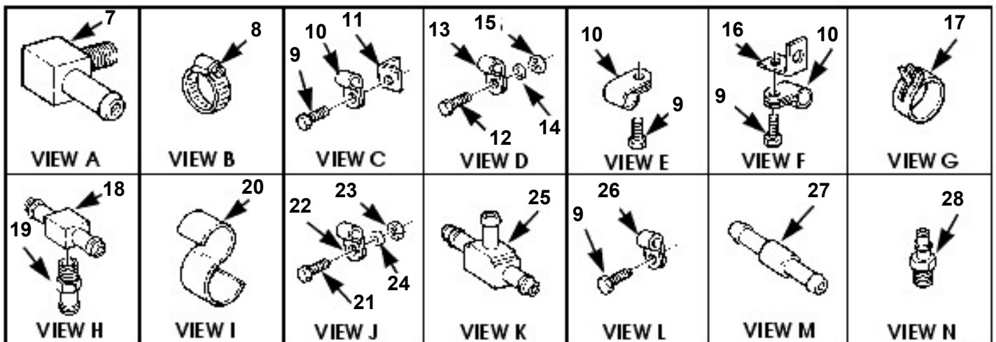
Front Axle Differential and Geared Hub Vent Lines.
