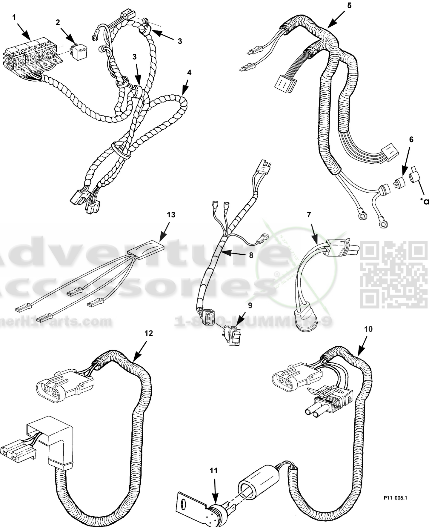
Wiring Harnesses, A/C-Heat.
