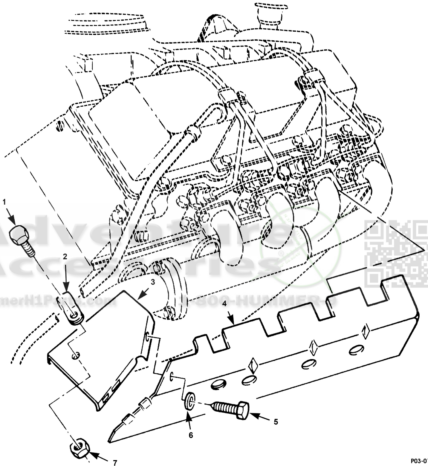
Exhaust Manifold Heat Shield.
