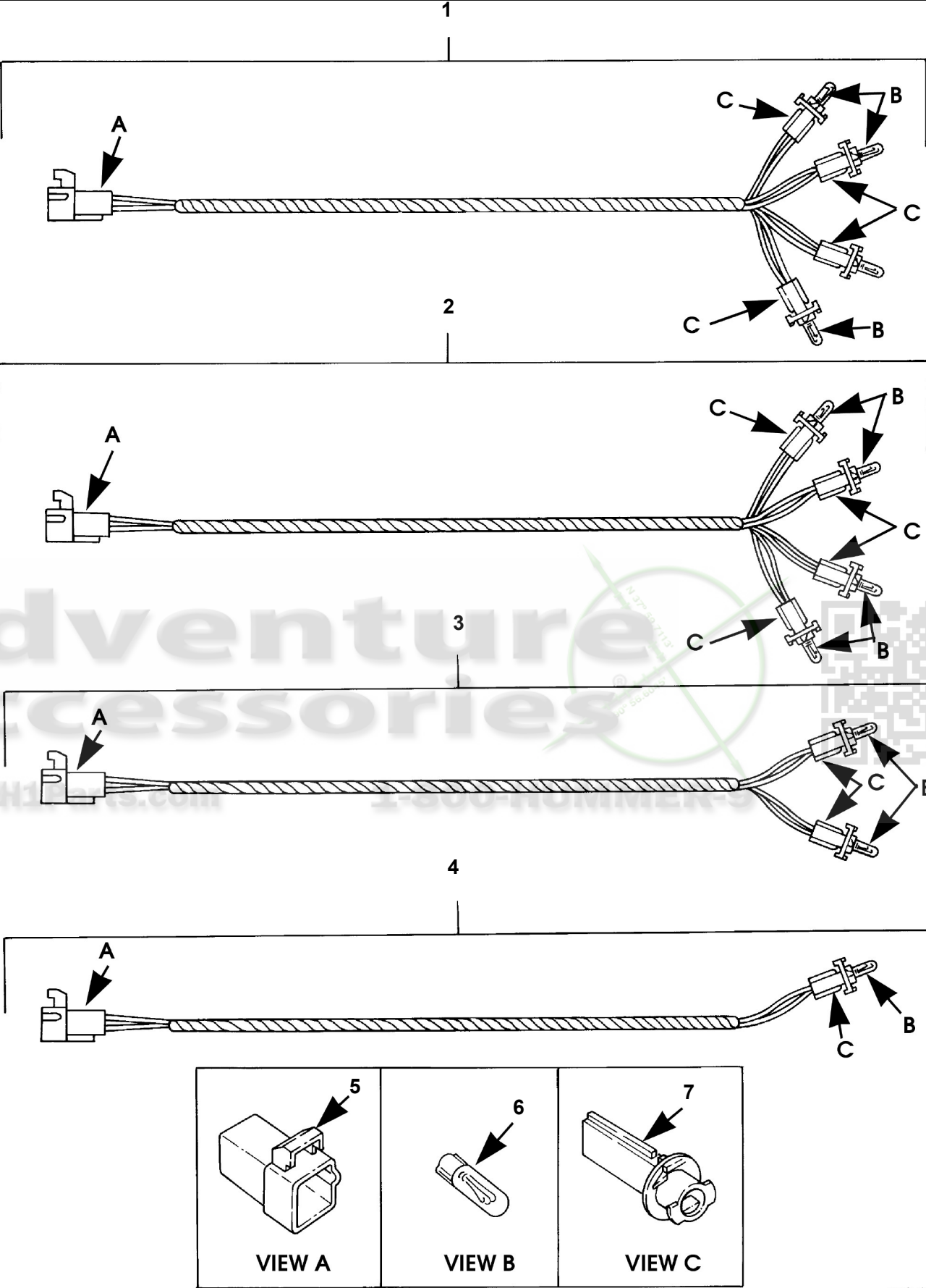
Instrument Panel Jumper Assemblies.
