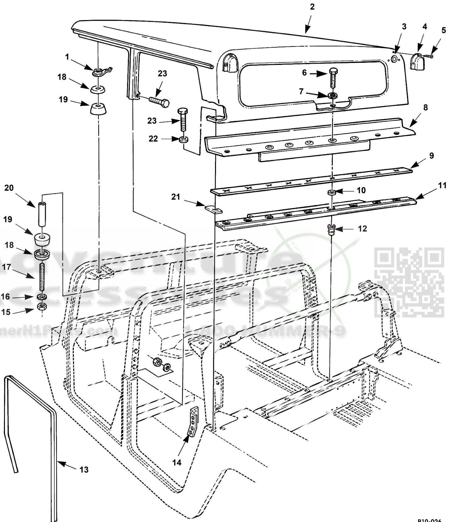
Four-Man Hardtop Assembly.
