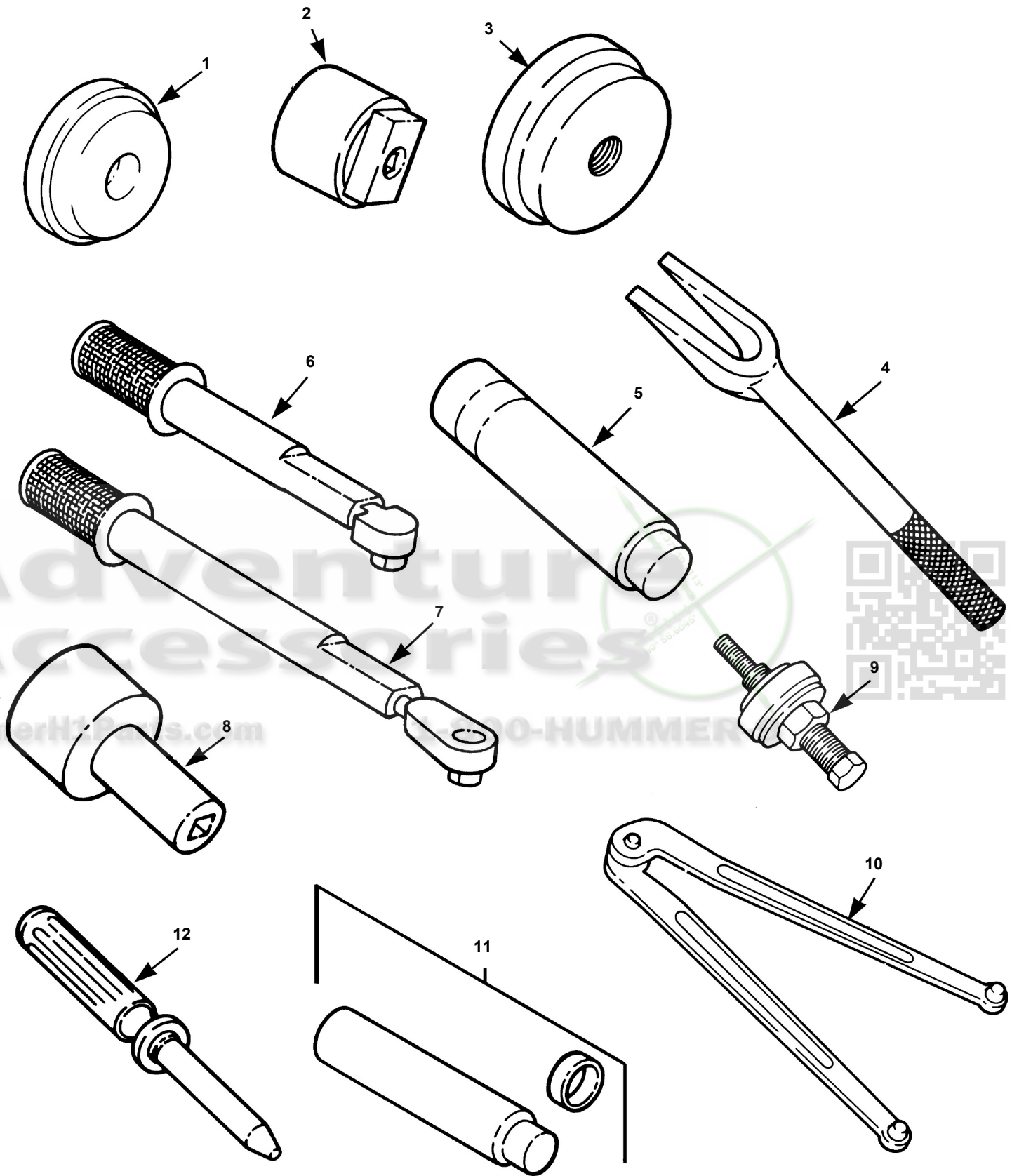
Special Tools, Geared Hub and Steering.
