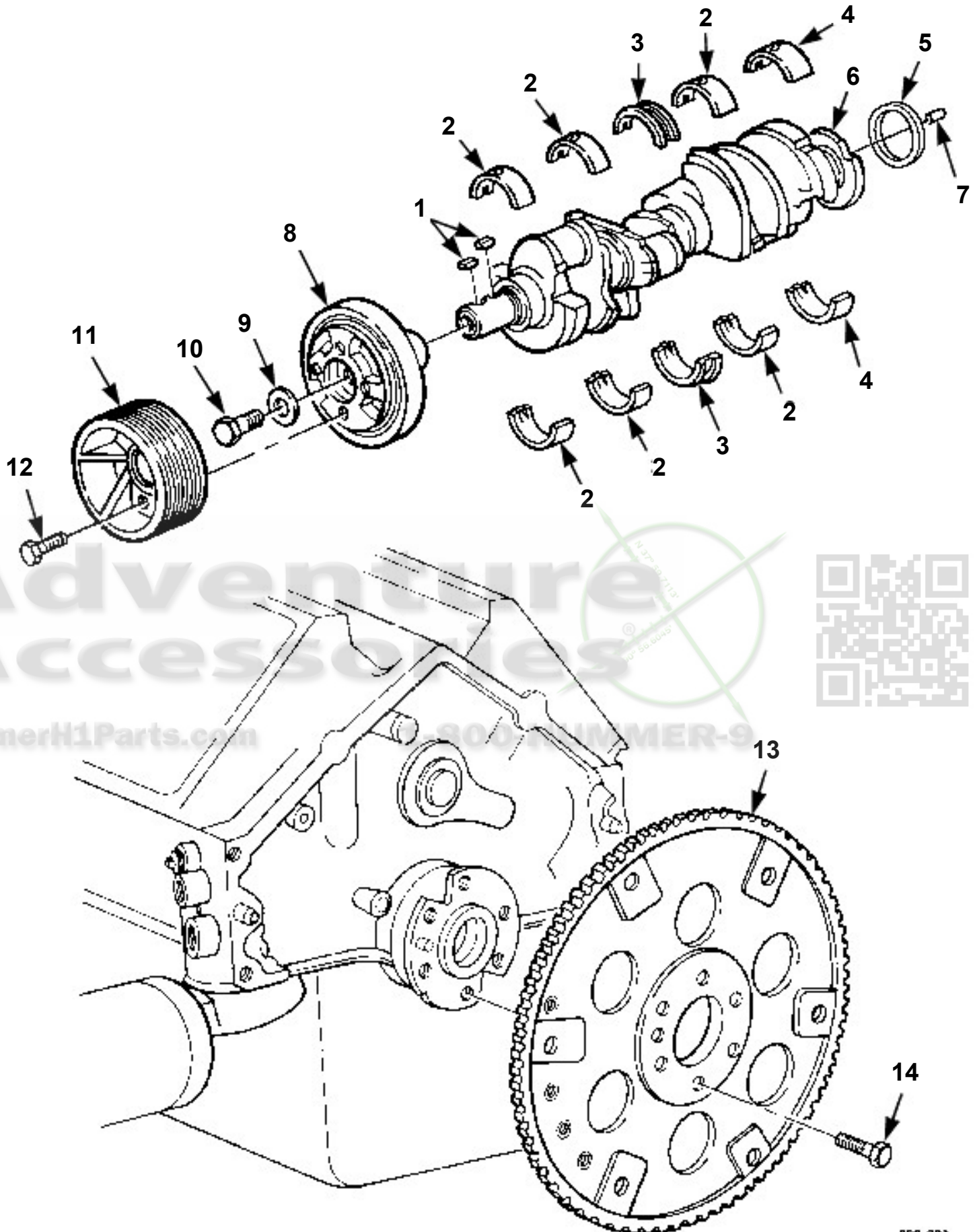
Crankshaft, Damper, Bearings, Pulley and Flywheel
