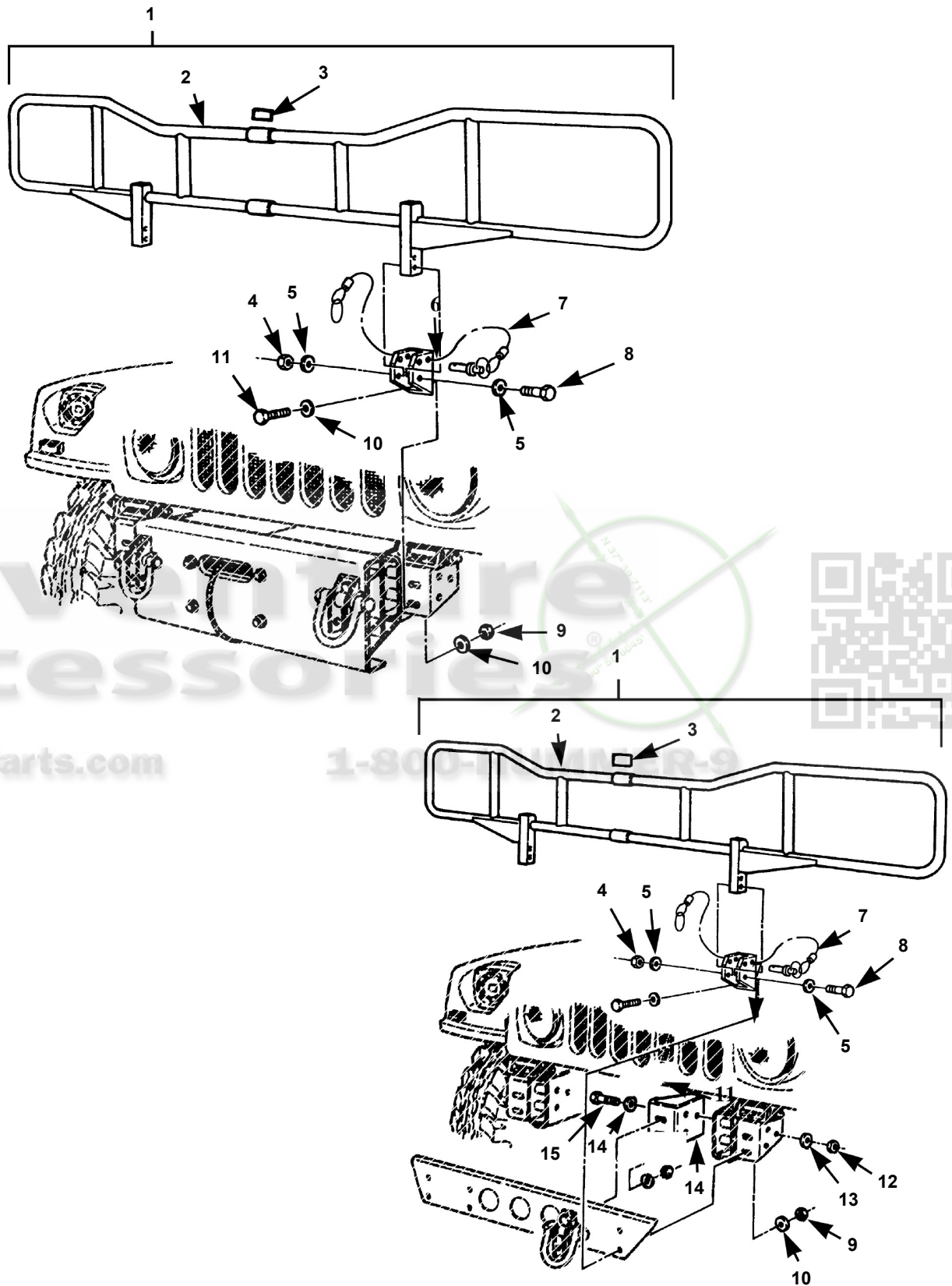
Brushguard Kit and Mounting Hardware.
