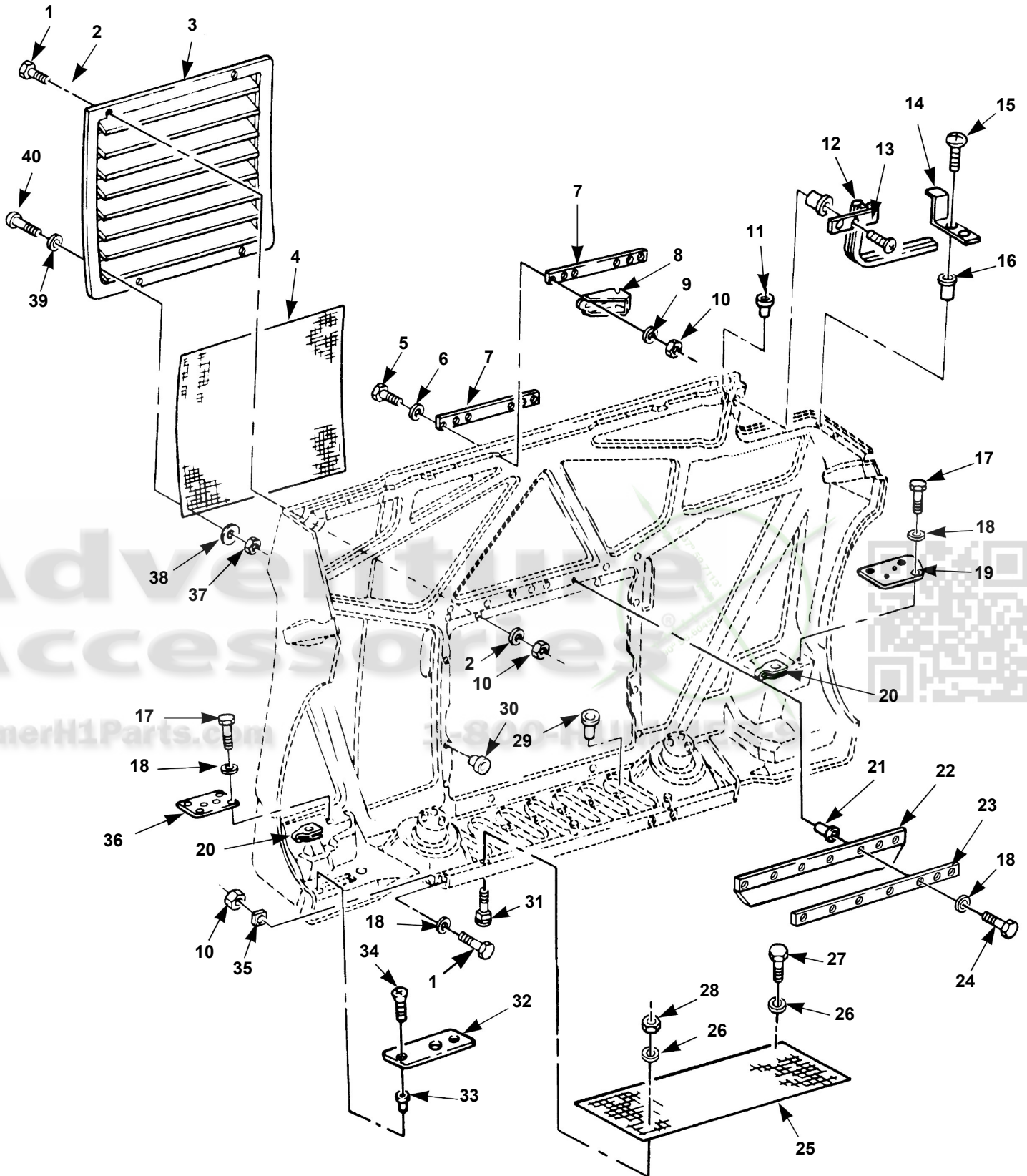
Hood Assembly. Grille, and Related Parts.
