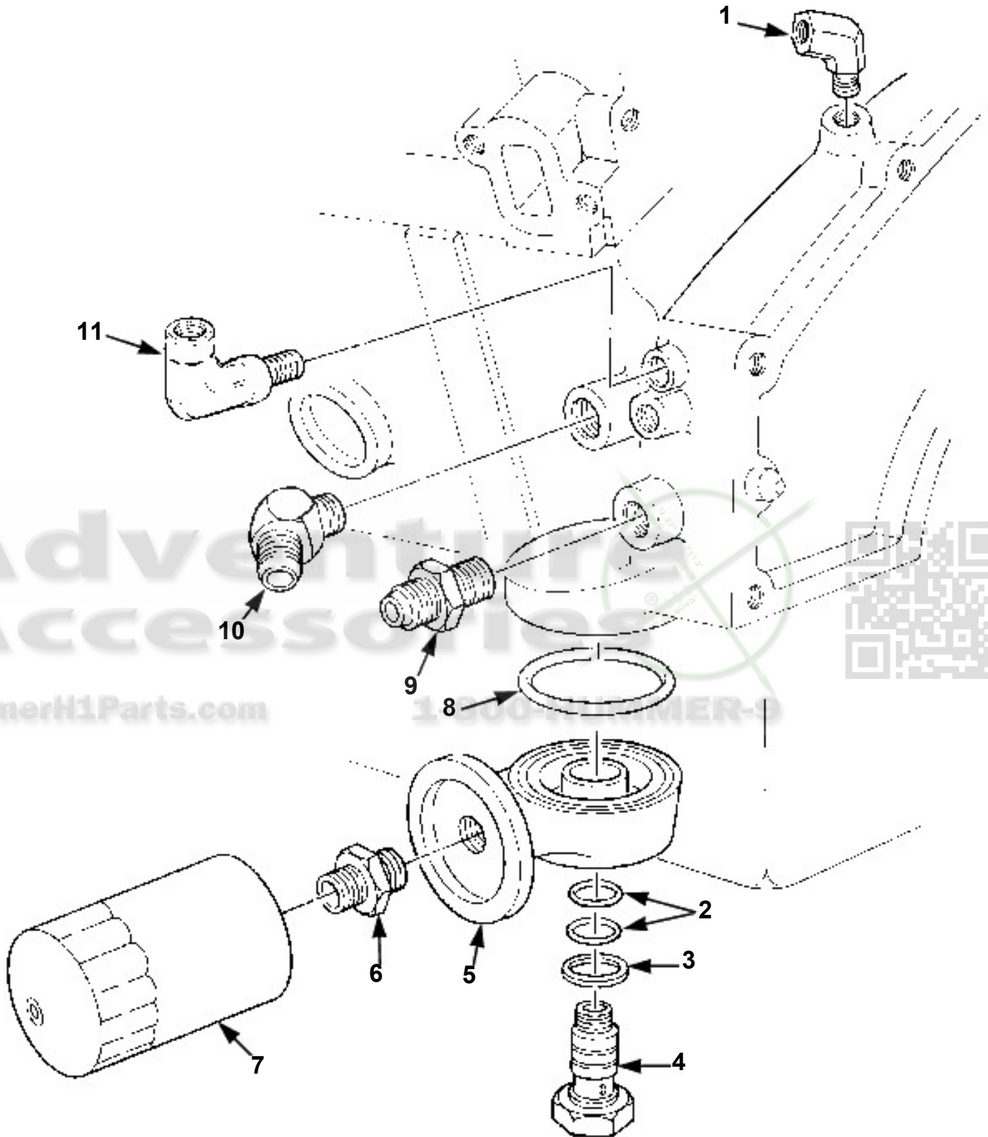
Oil Filter, Adapter, and Oil Line Fittings
