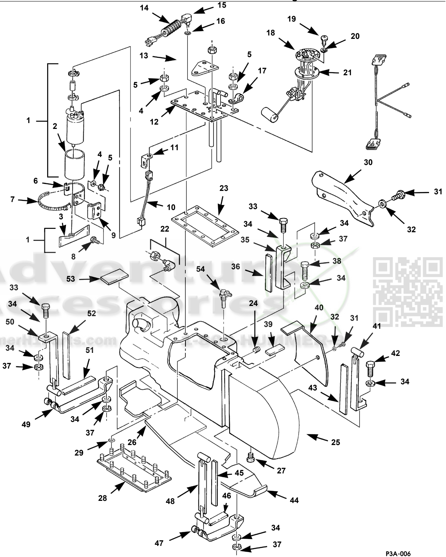
Fuel Tank Assembly and Mounting Straps.
