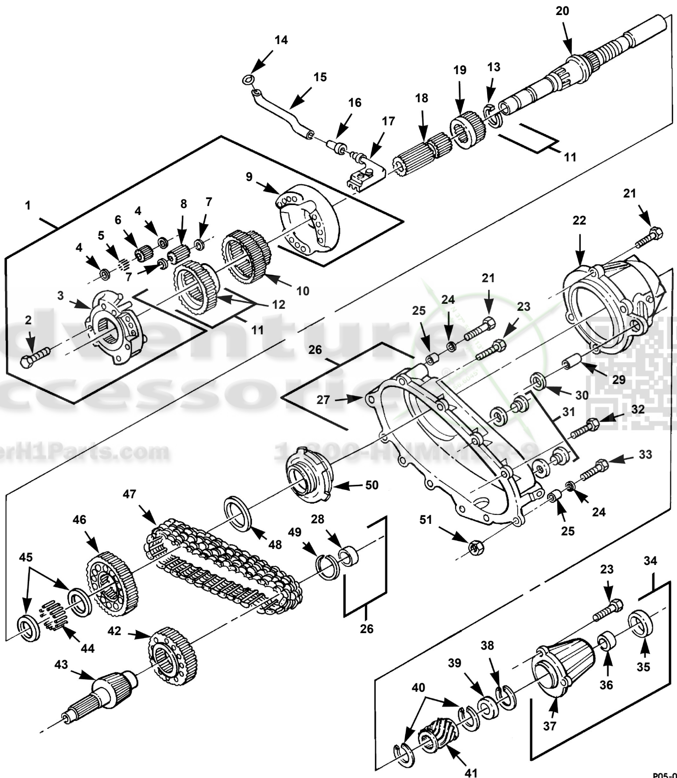
Transfer Case Assembly, Rear Half.
