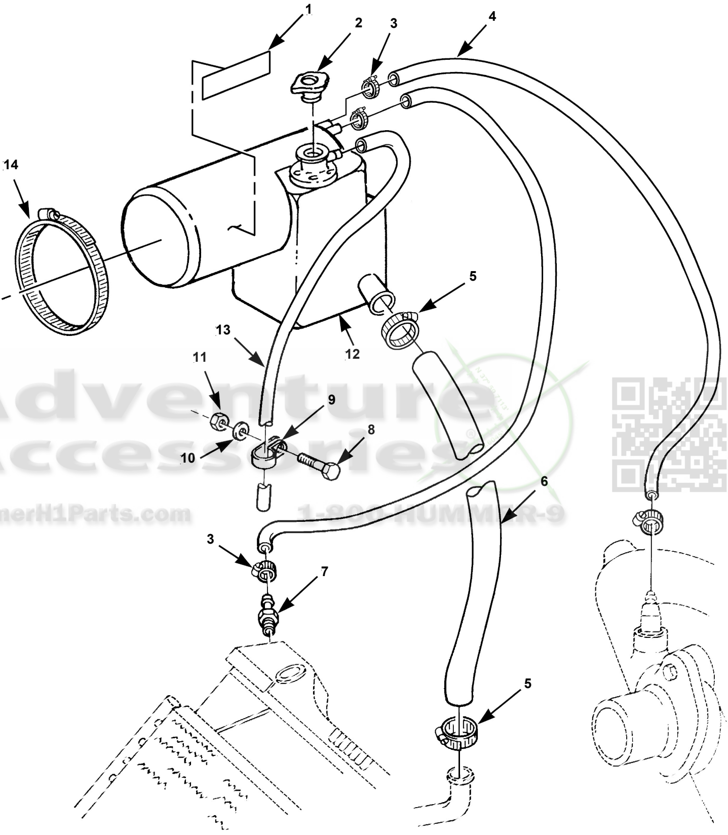
Surge Tank and Related Parts.
