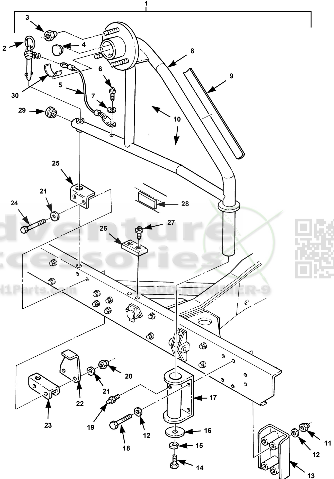
Swing-Away Spare Tire Carrier.
