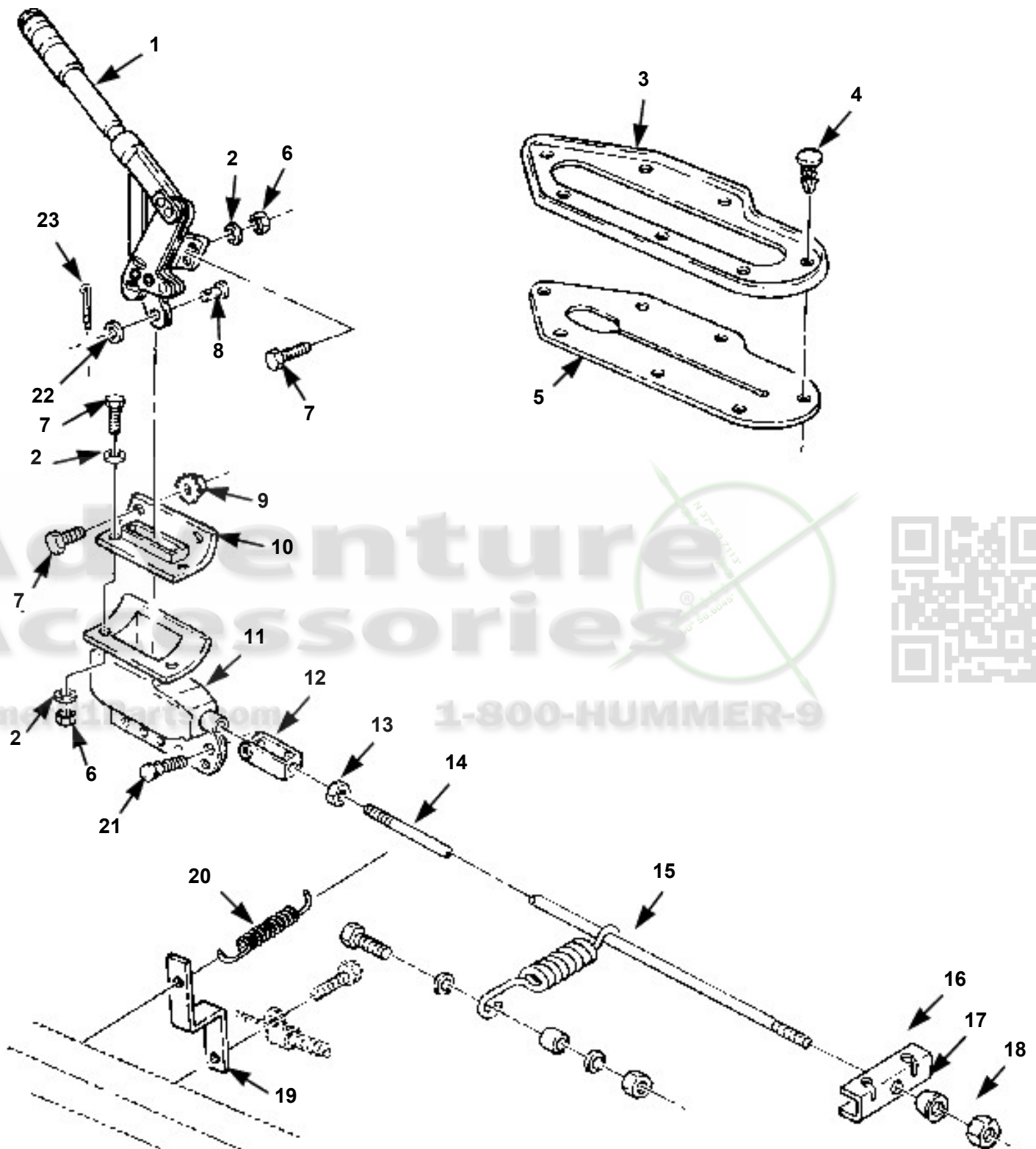
Parking Brake Hand Lever and Rod.
