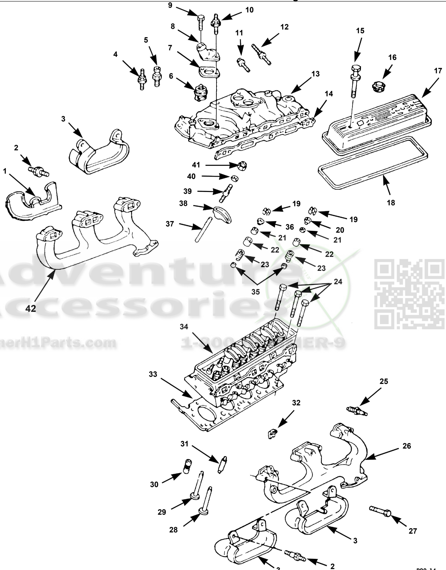
Cylinder Head, Manifolds and Components
