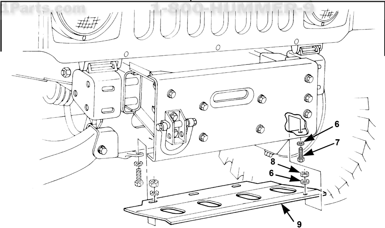
Underbody Protection Skid Plates.
