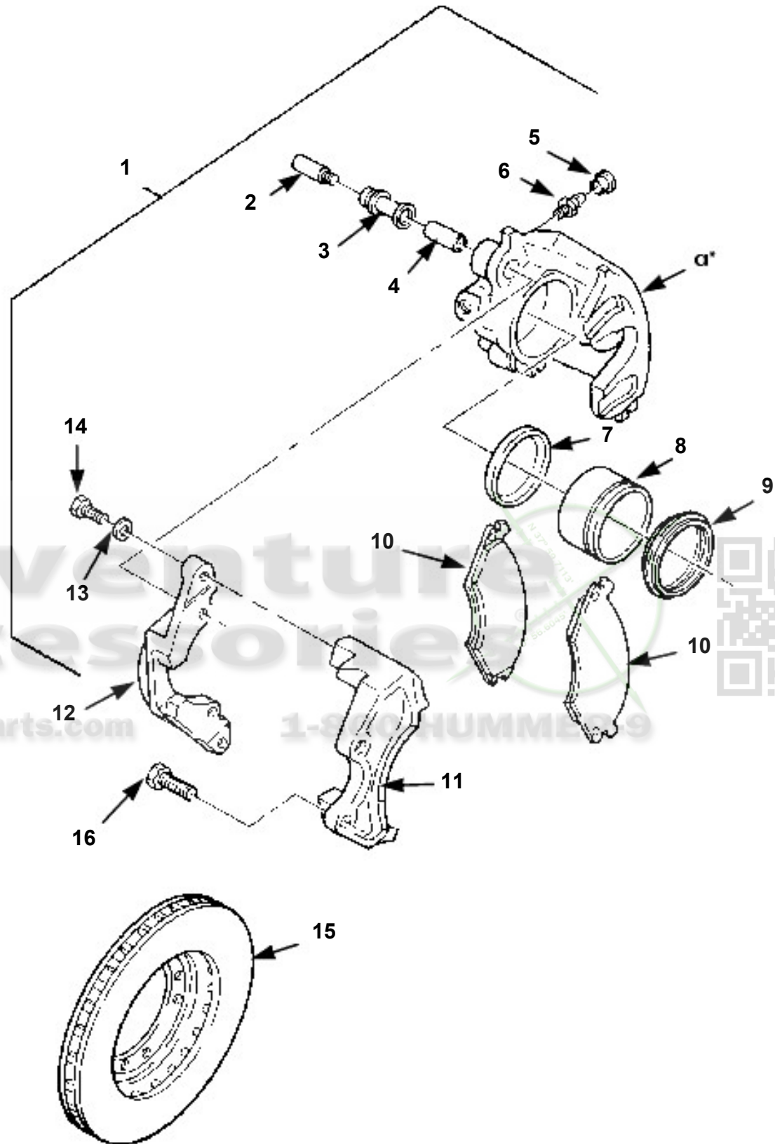
Service Brake Caliper Assembly and Rotor.
