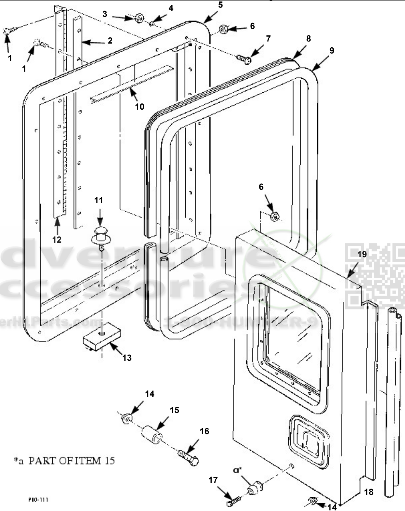
Station Wagon Rear Doors (Graphic 1 of 2)
