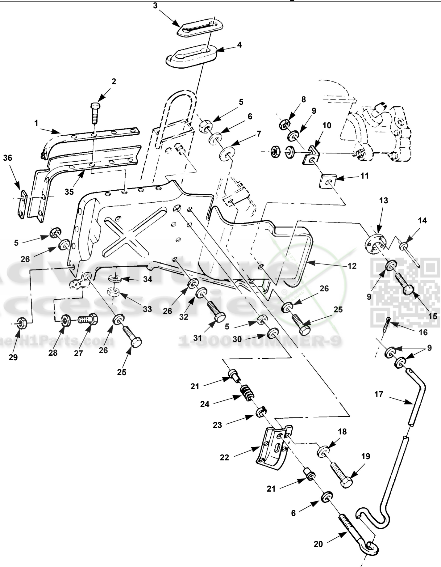
Left Hand Splash Shield and Hood Prop Rod.
