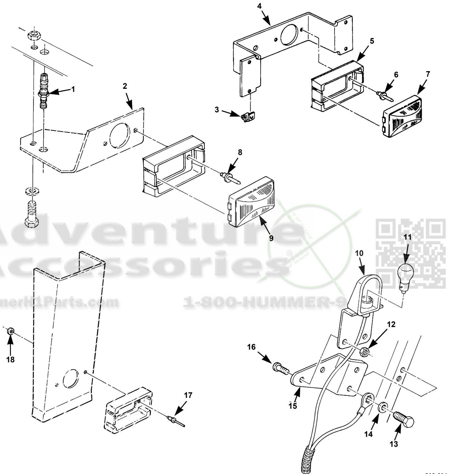
Interior Courtesy Lights, Underhood Light, and Door Jamb Switch.
