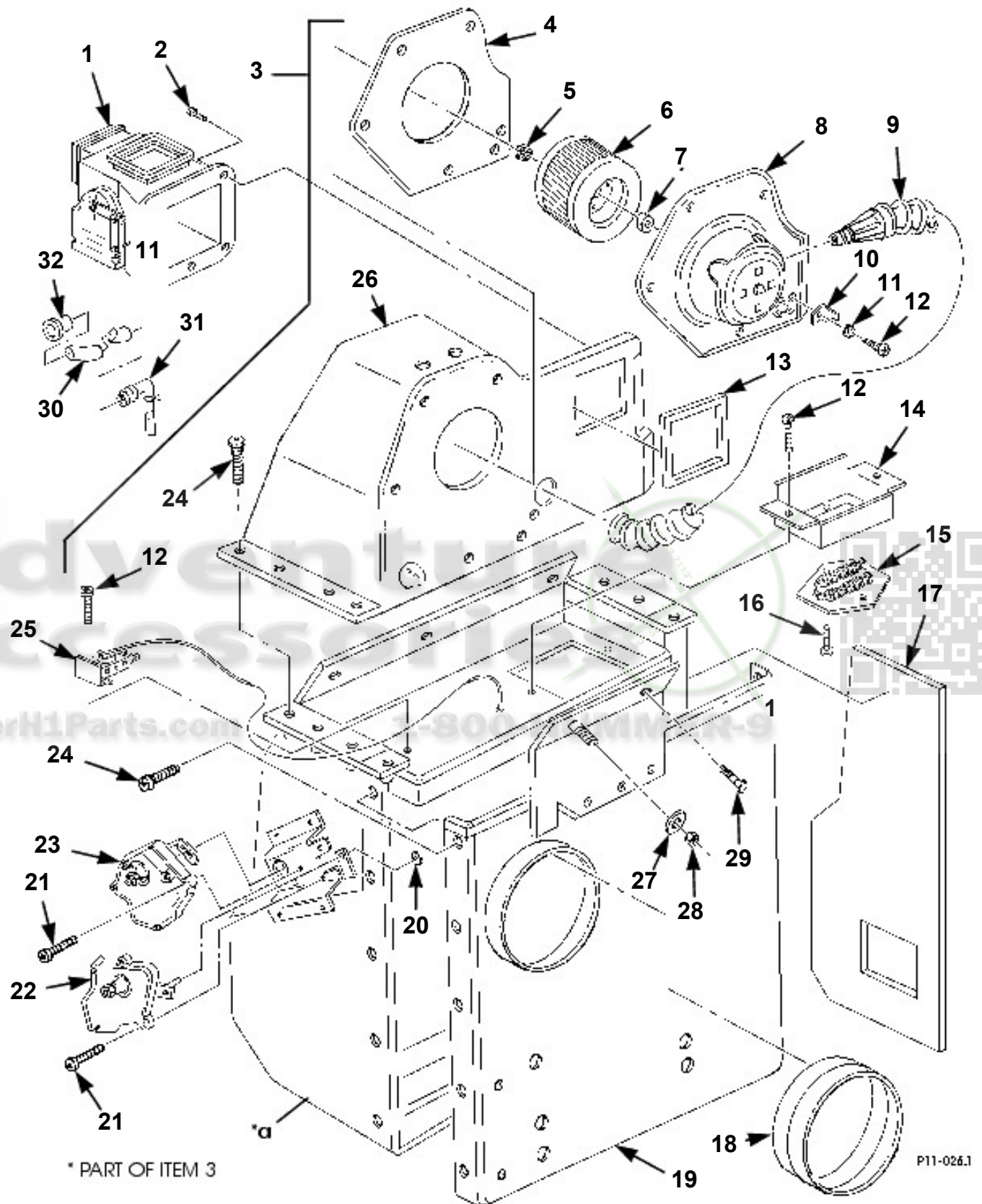
Main A/C-Heat Unit.
