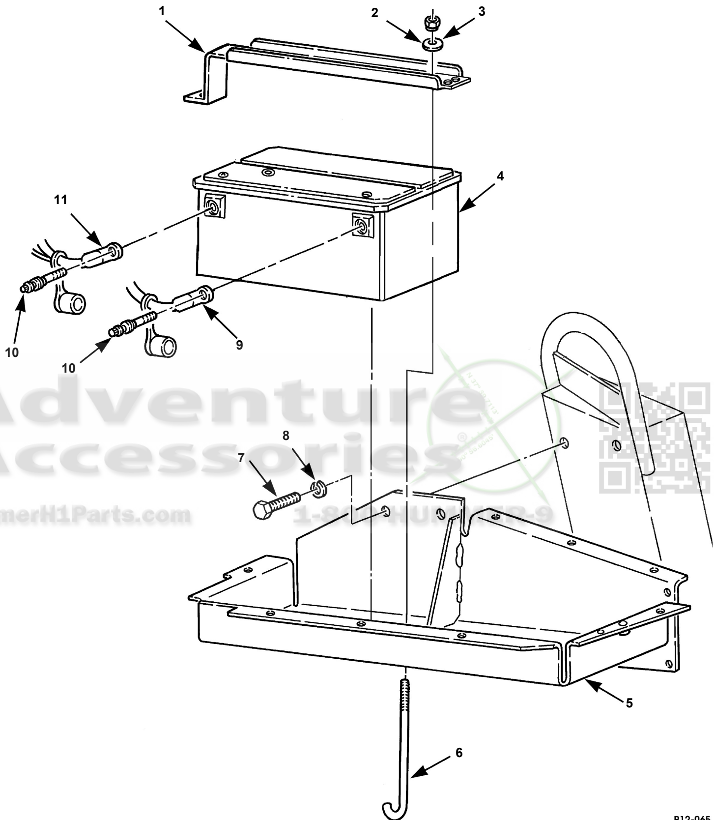
Battery, Cables, and Mounting Hardware.
