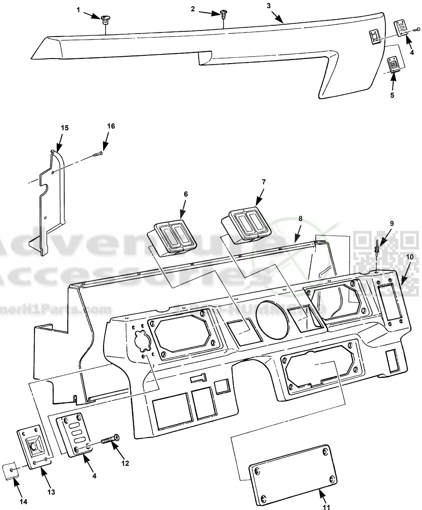
Instrument Panel Assembly, Dash Trim, and Crash Pad
