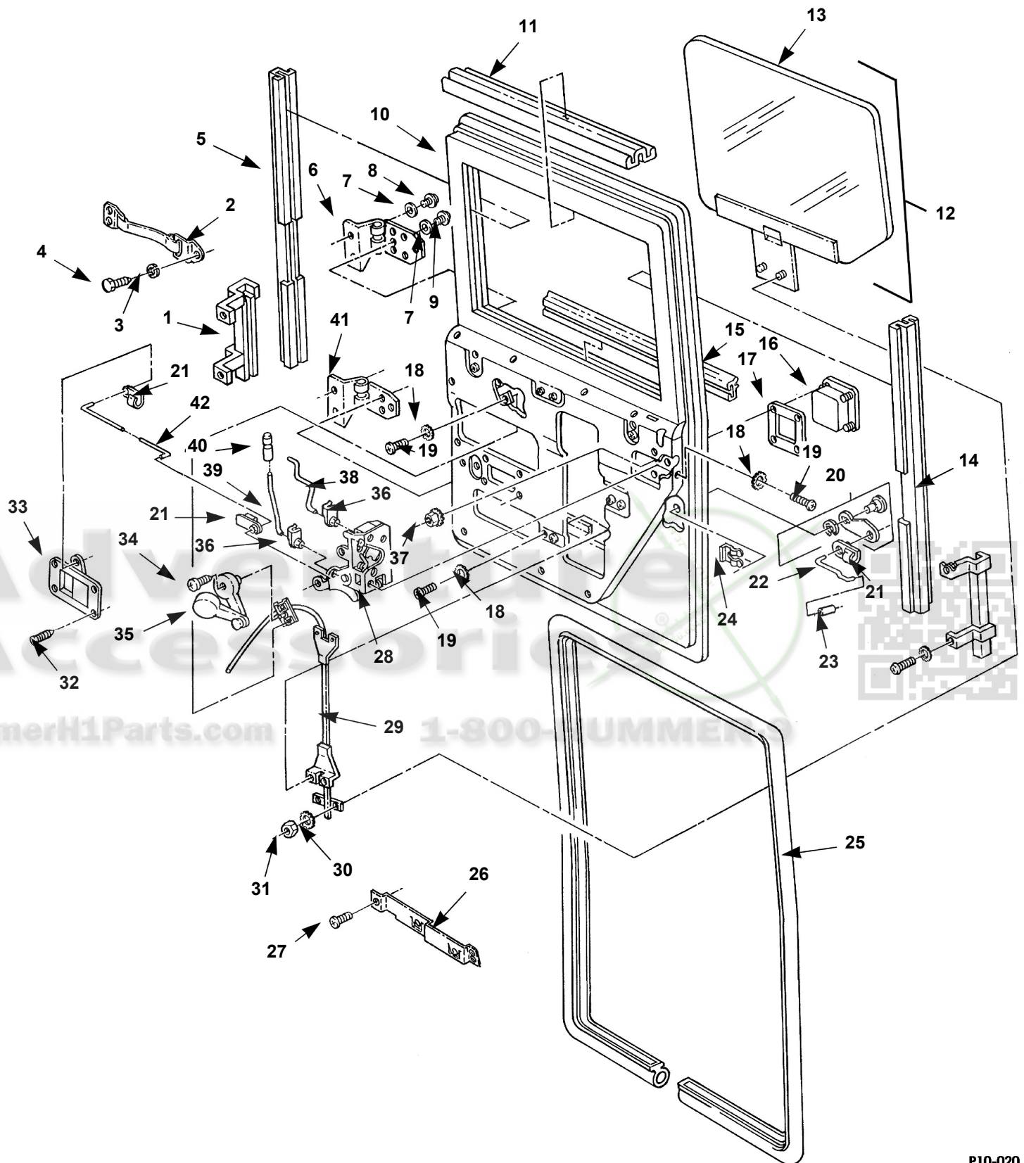
Front Door Assembly.
