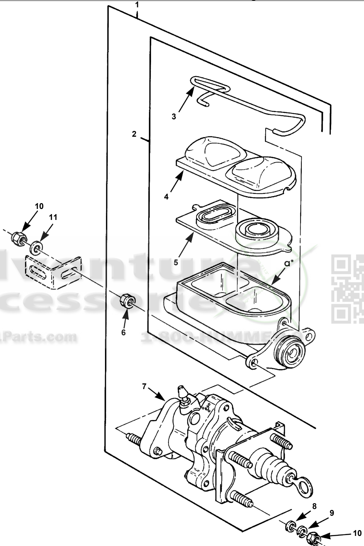
Master Cylinder Assembly and Hydro-Booster.
