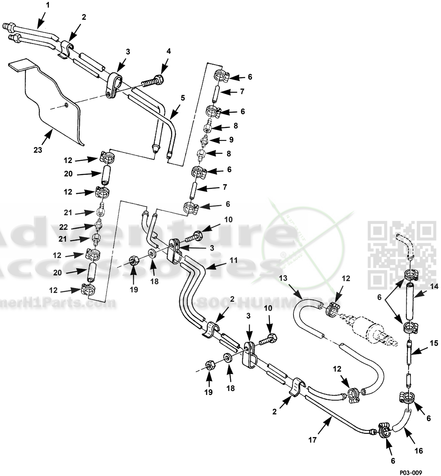
Fuel Tank Supply and Return Lines.
