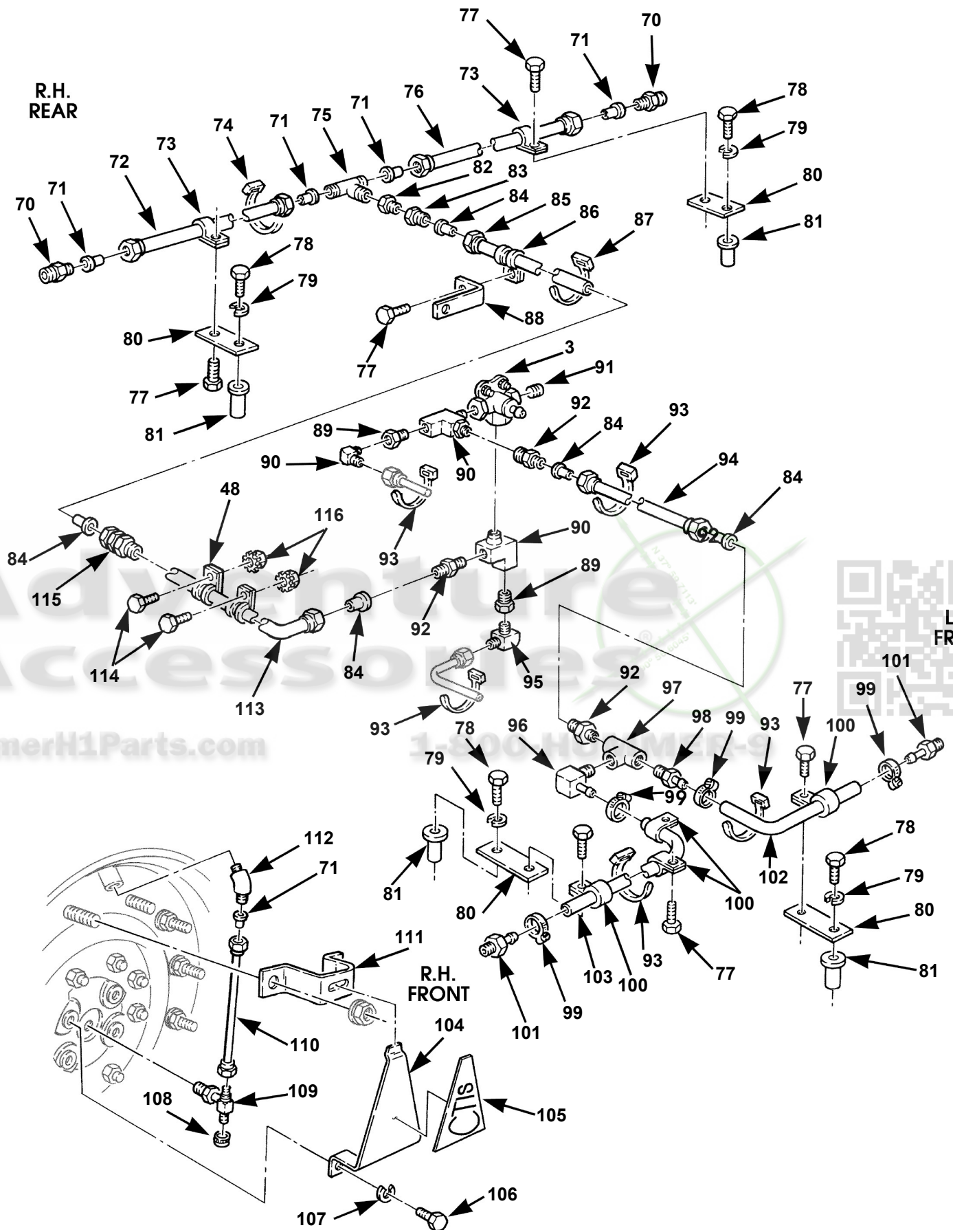
Central Tire Inflation System (Graphic 3 of 3)
