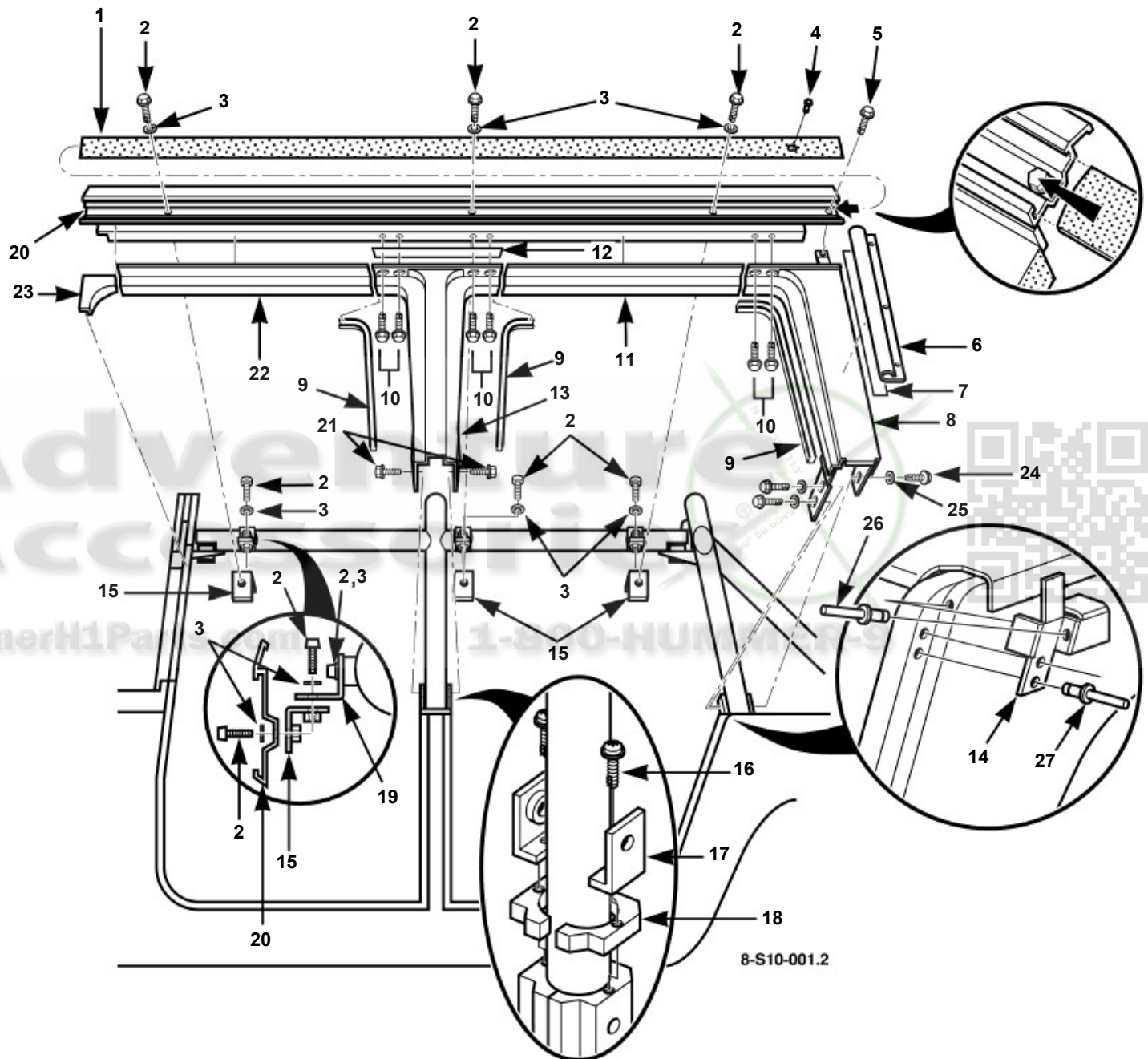
Support Structure, Soft Top, Model 90
