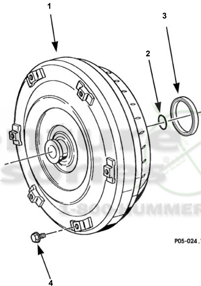
Torque Converter and Oil Pump
