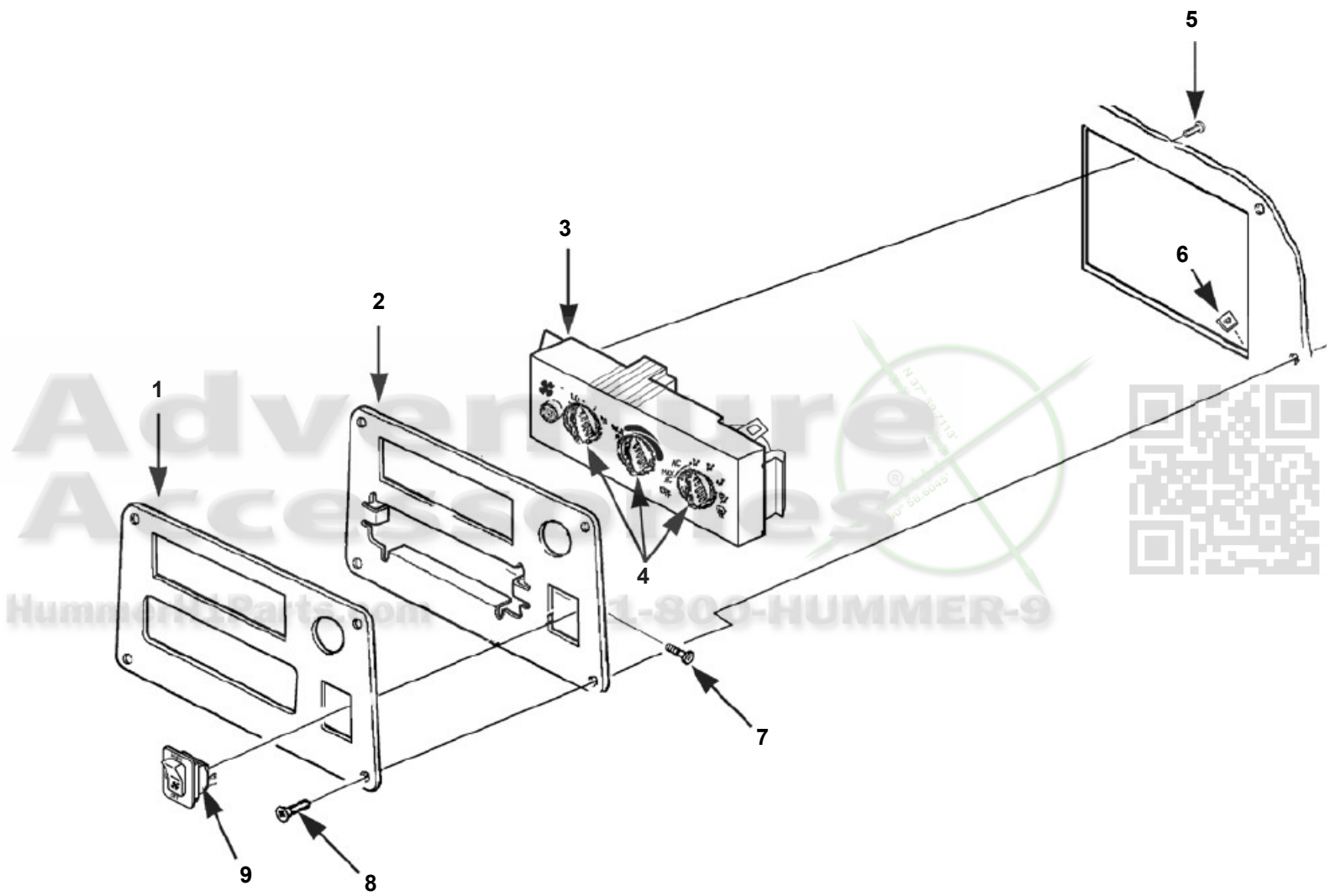
Climate Control Panel
