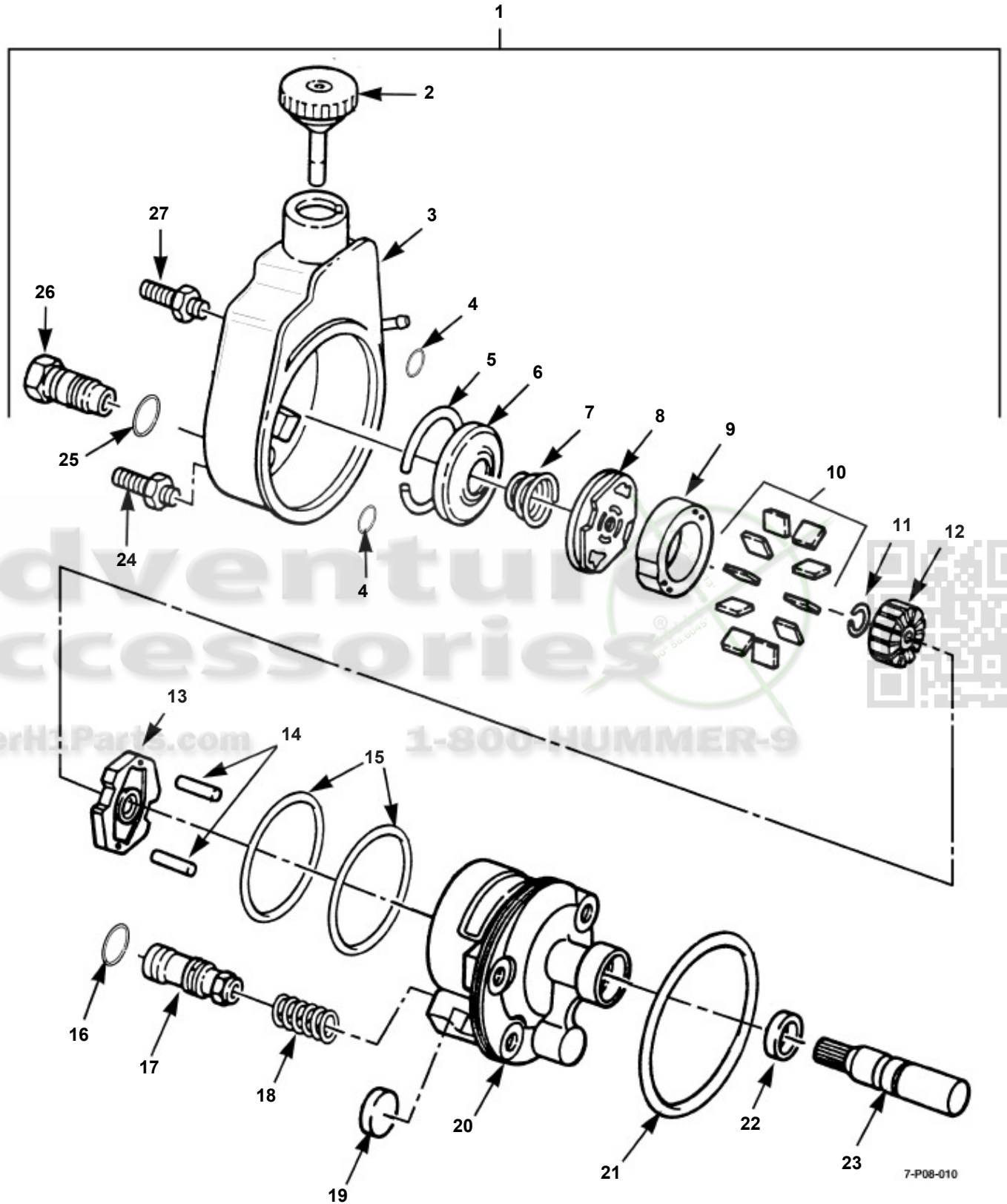
Power Steering Pump
