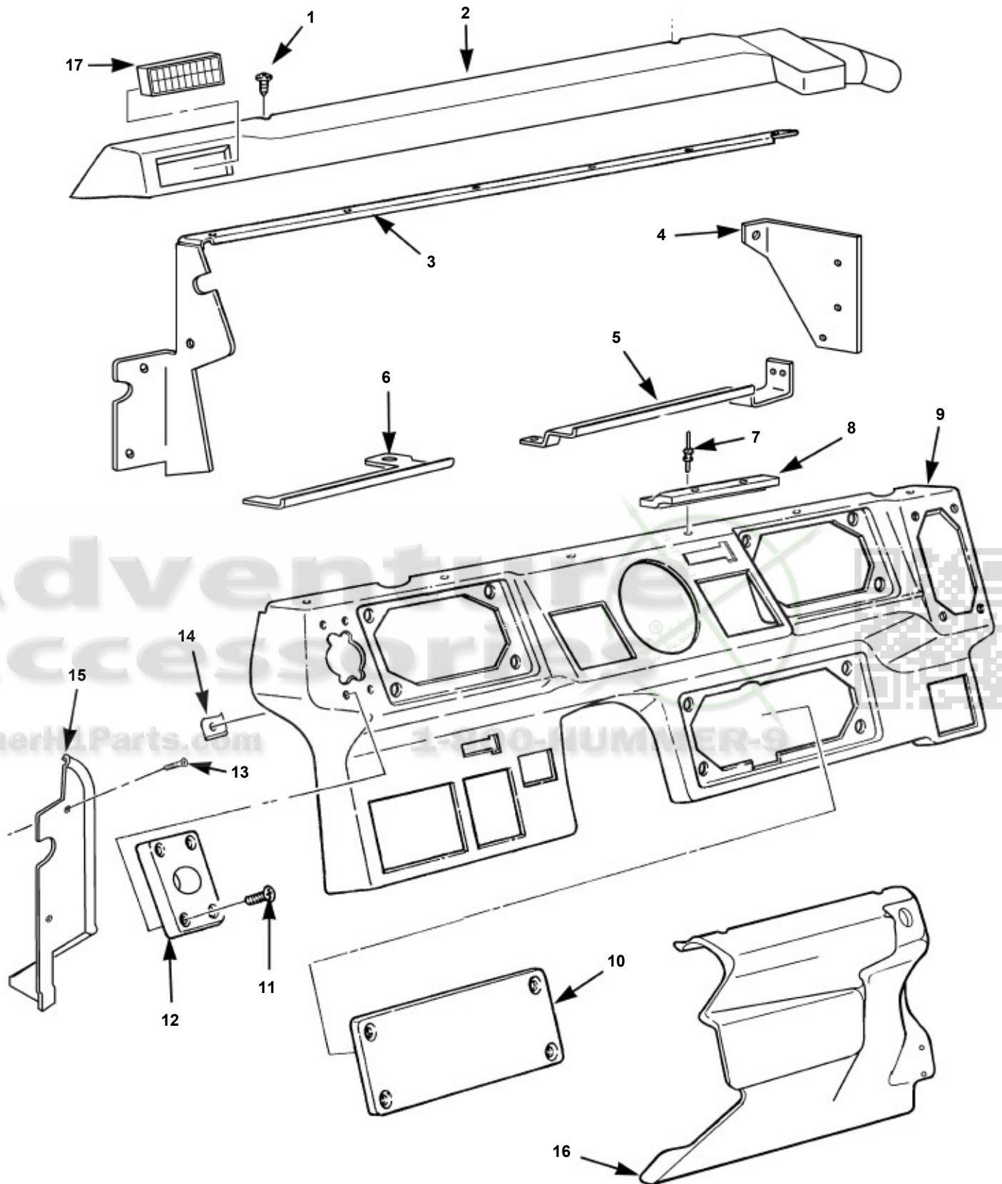
Instrument Panel Assembly, Dash Trim, Crash Pad, and Mounting Hardware
