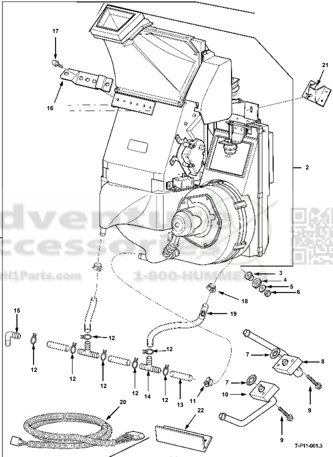
Main A/C-Heat Unit
