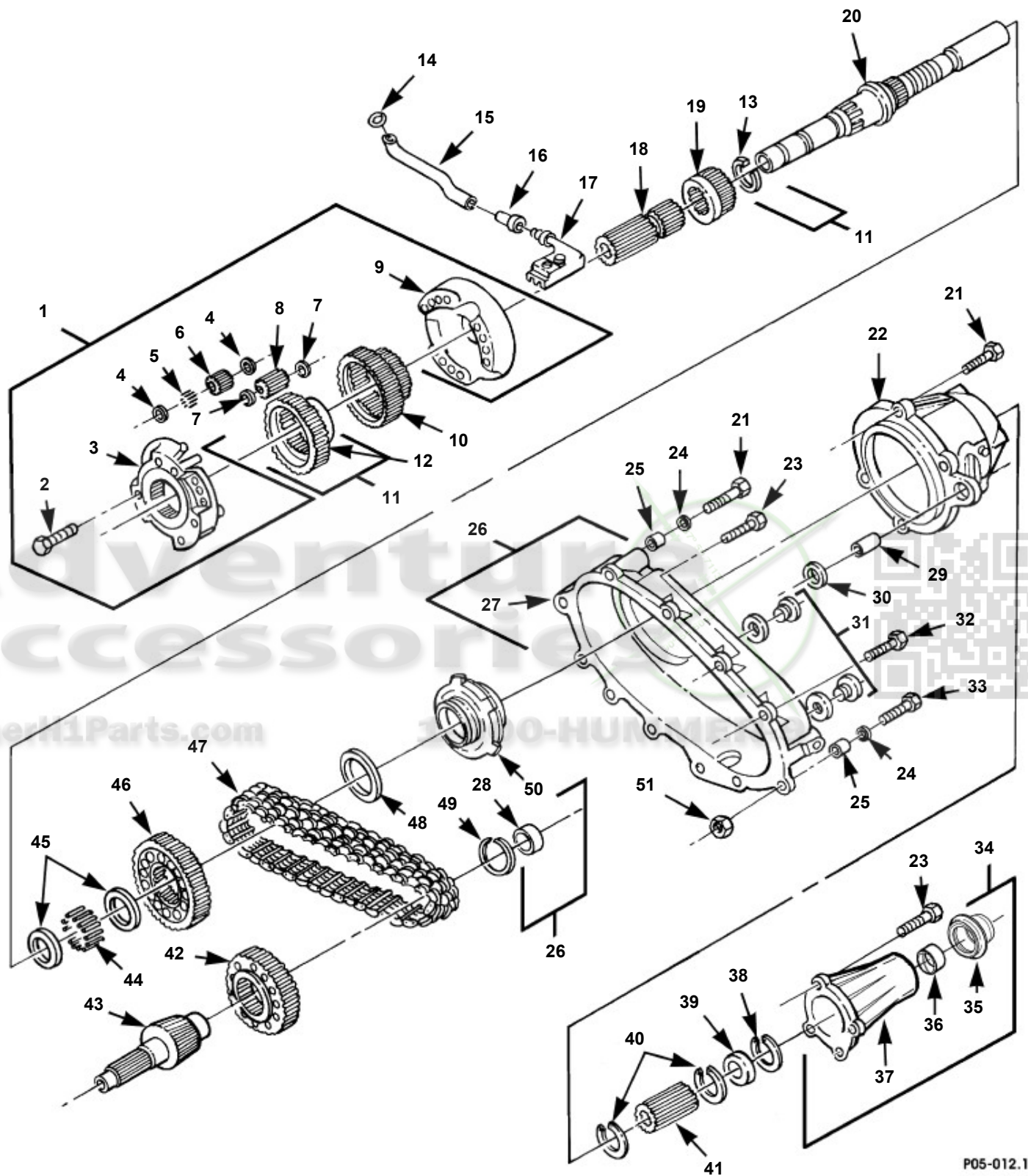
Transfer Case Assembly, Rear Half
