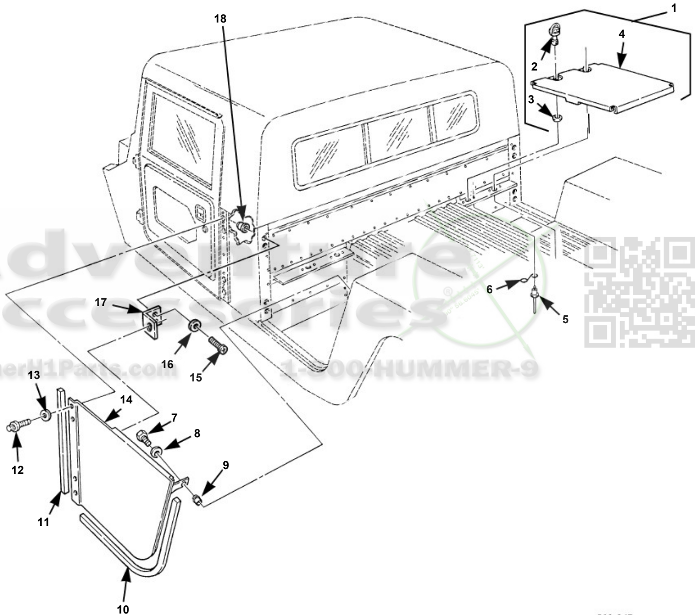
Fixed Door, Footwell Cover, and Related Parts, Two-Passenger Enlarged Cab, Model 89
