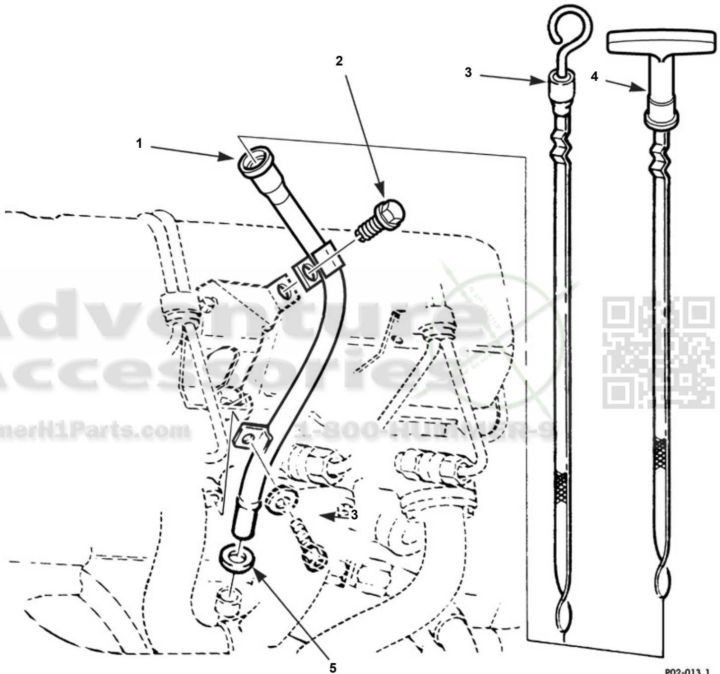
Engine Oil Dipstick and Tube Assembly
