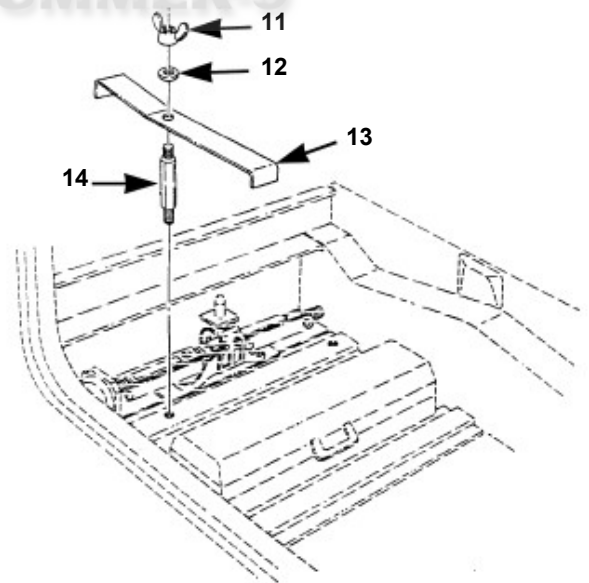
Reflective Triangle Warning Device, Jack Assembly, and Mounting Hardware
