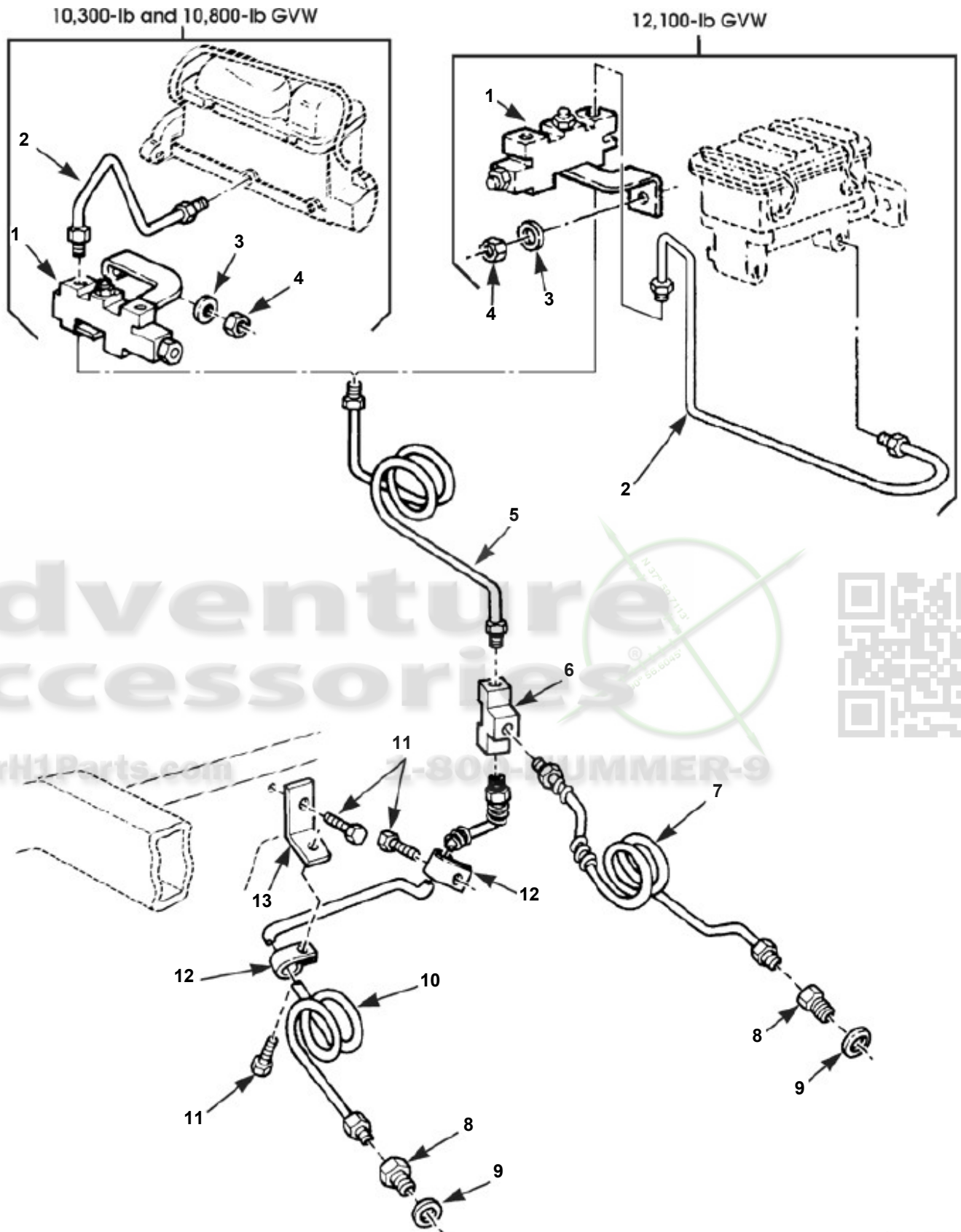
Front Service Brake Lines and Proportioning Valve, 10,300-lb, 10,800-lb, and 12,100-lb GVW
