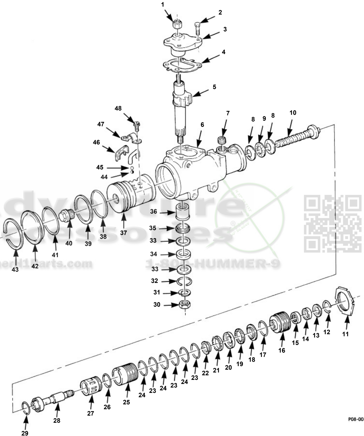
Power Steering Gear Assembly
