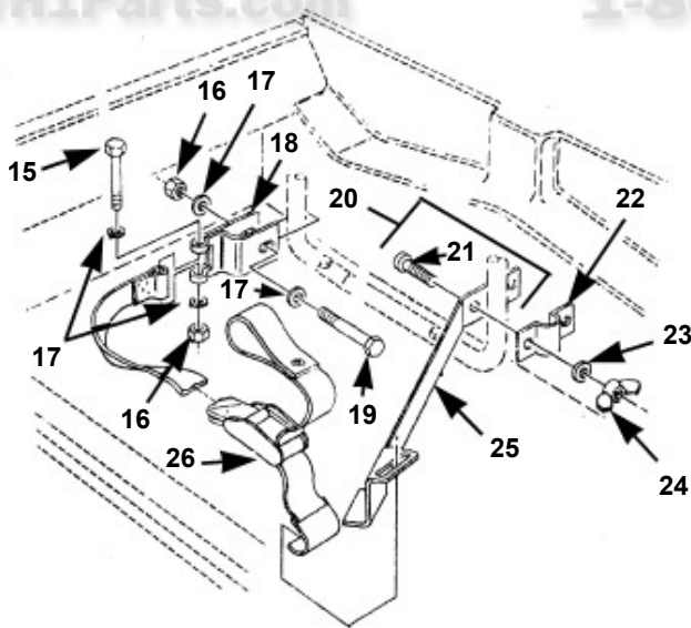
Reflective Triangle Warning Device, Jack Assembly, and Mounting Hardware
