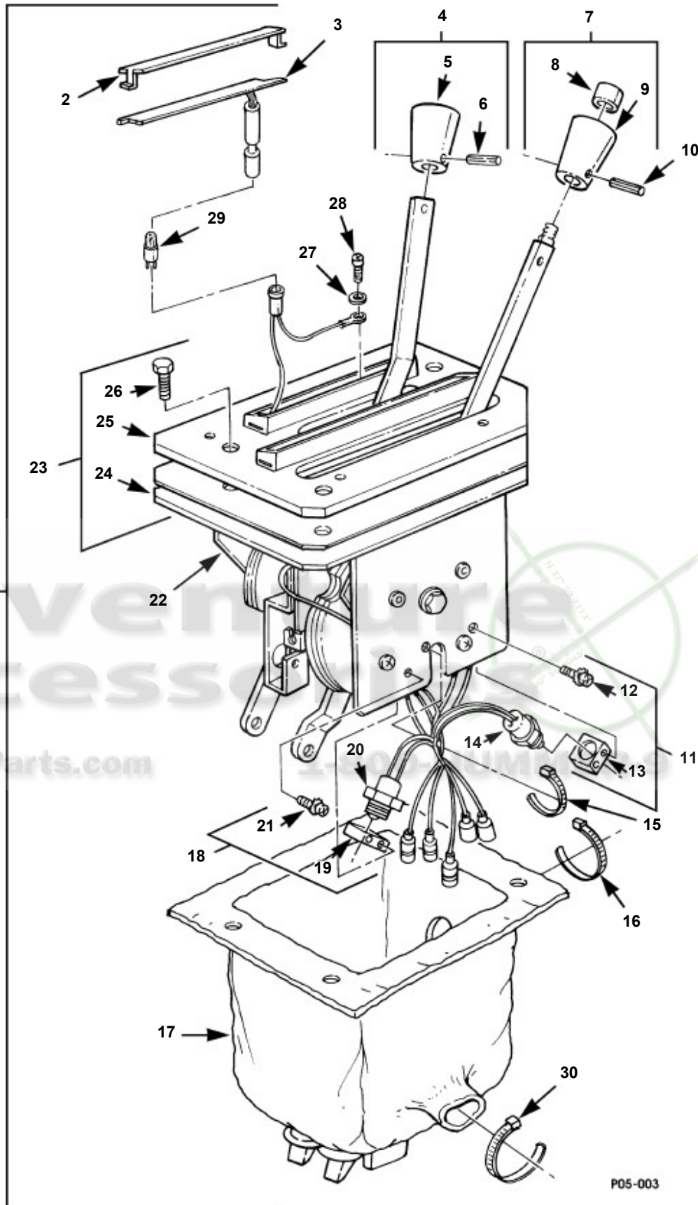
Transmission and Transfer Case Control Assembly and Neutral Star Switch
