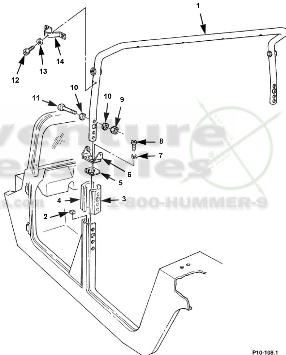
B-Bar, Two-Passenger Enlarged Cab, Model 89
