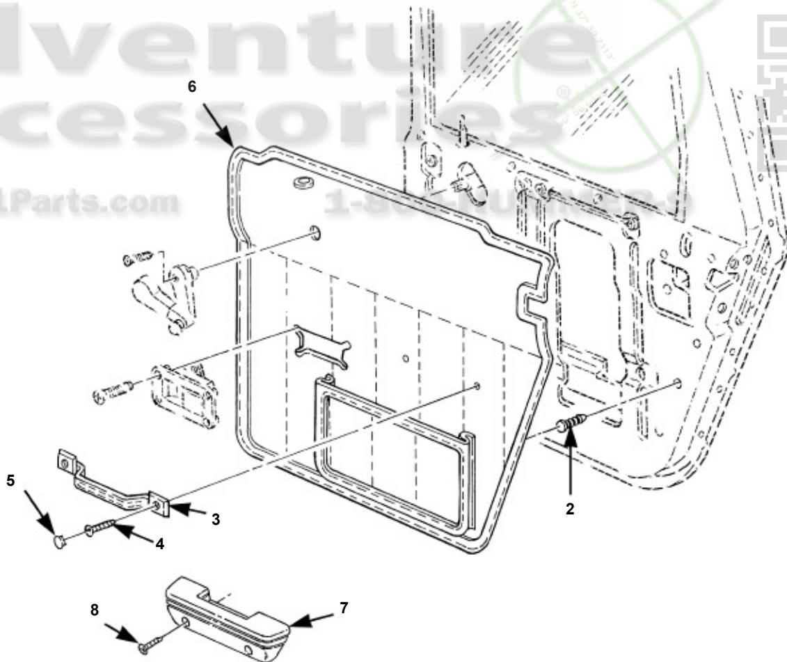
Panel Assembly Door Trim
