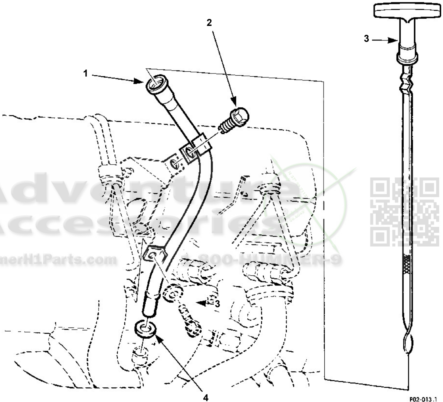
Oil Dipstick and Tube Assembly, Engine.
