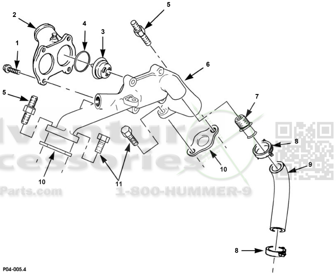
Thermostat, Water Crossover, and Attaching Hardware
