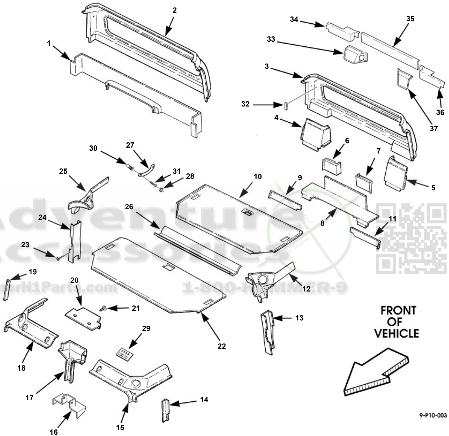
Headliner, Roof Trim, Front and Rear Side Trim, Grab Handles, and Mounting Hardware (Delco Standard Stereo System)
